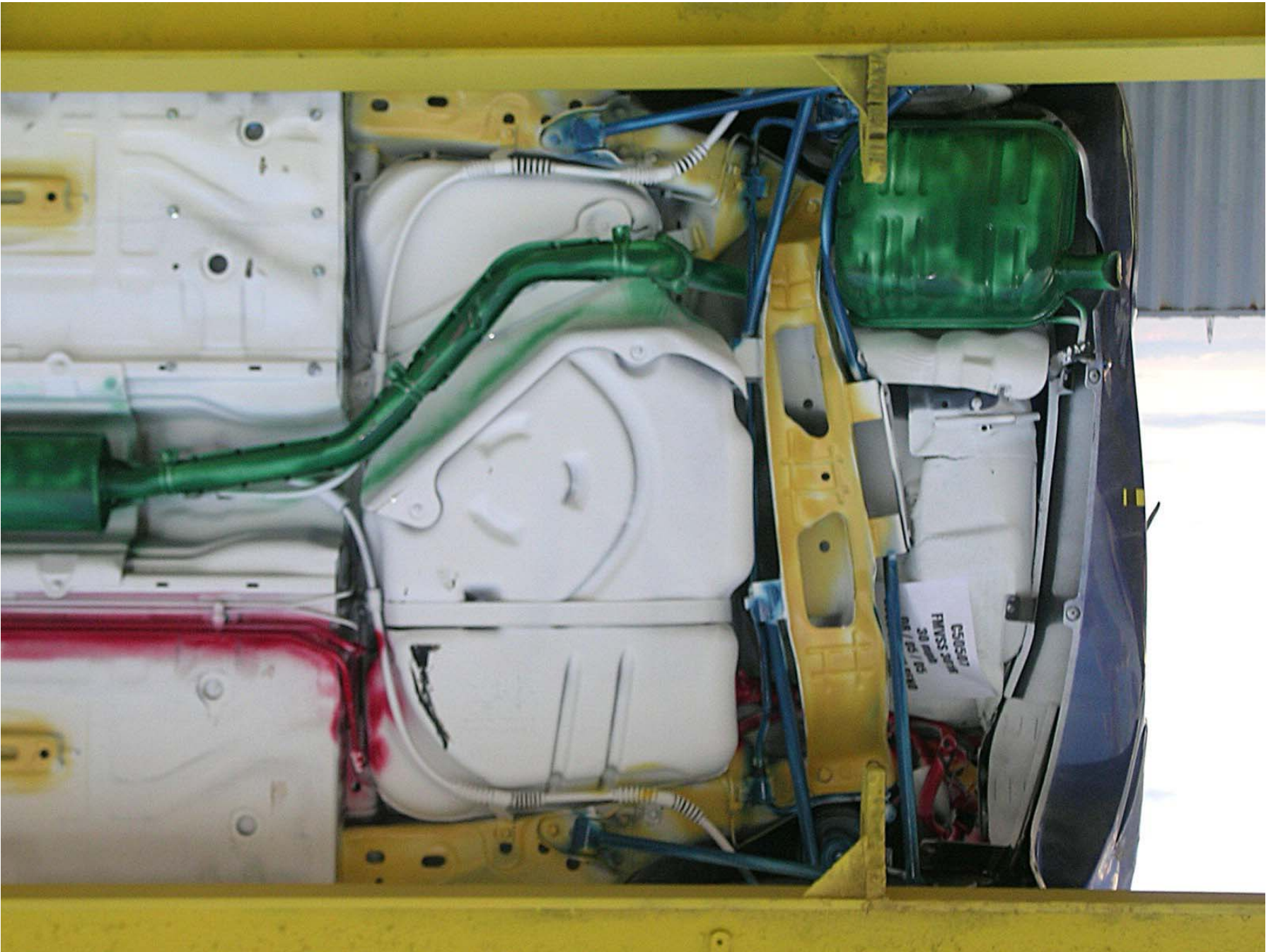
Figure A-20: Post-Test Rear Underbody
