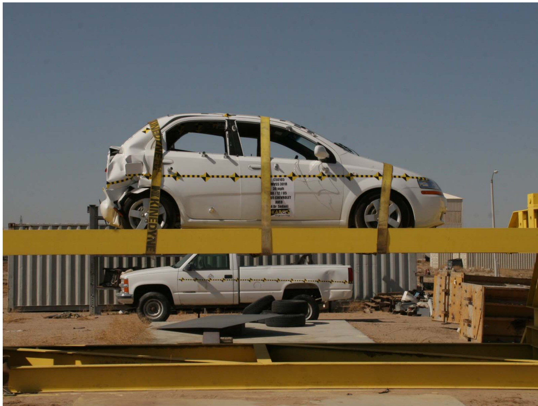
Figure A-21: Vehicle on Rollover Device at 0°
