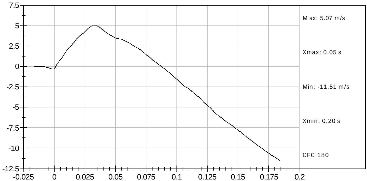
PENDULUM DECELERATION (m/s) vs TIME (s)
