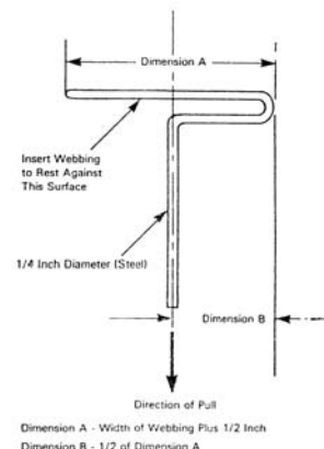
Figure 5. - Webbing Tension Pull Device
