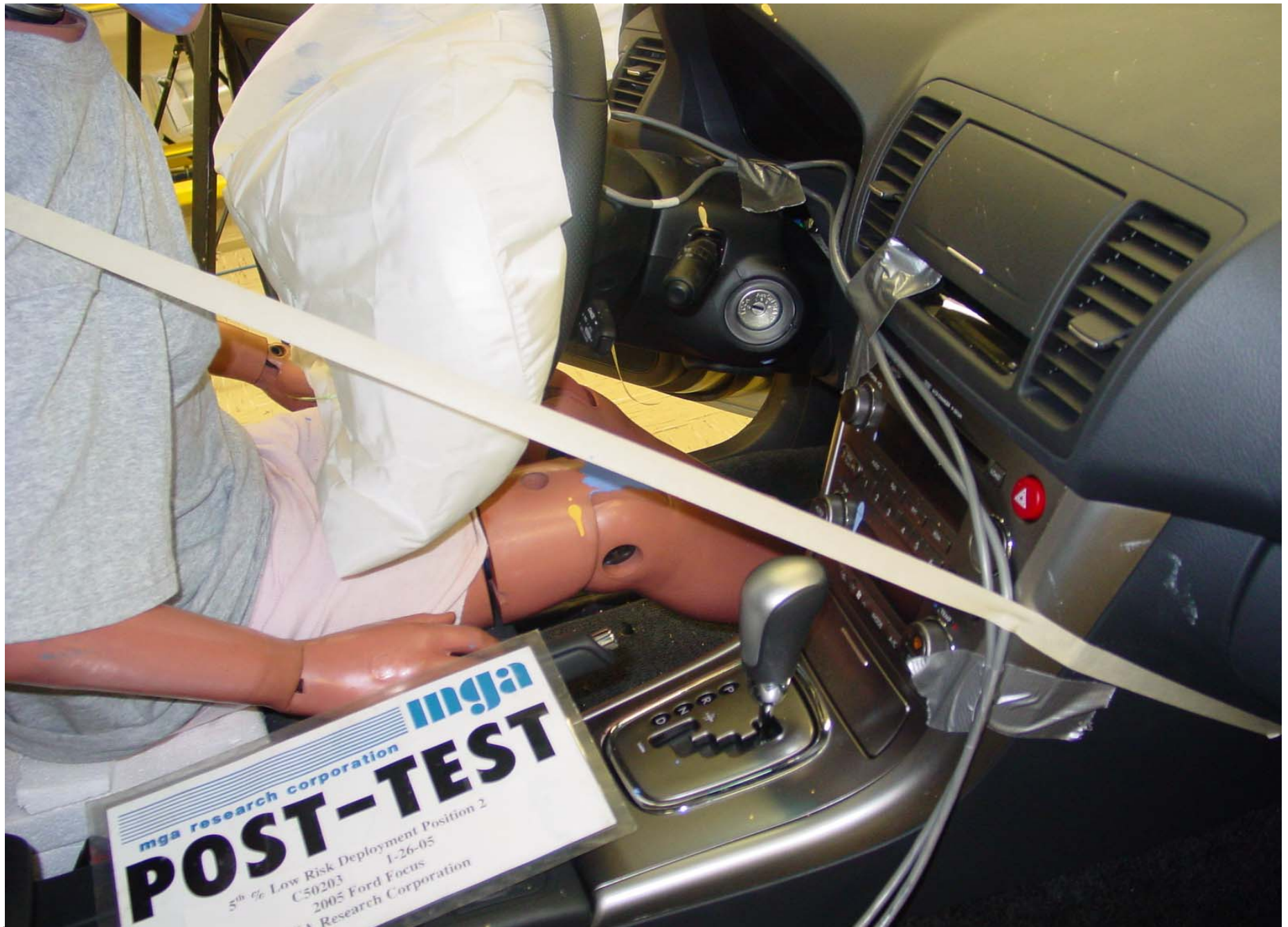
Post-Test 5th Fem. P2 Driver Dummy Right Side Knee Position View
