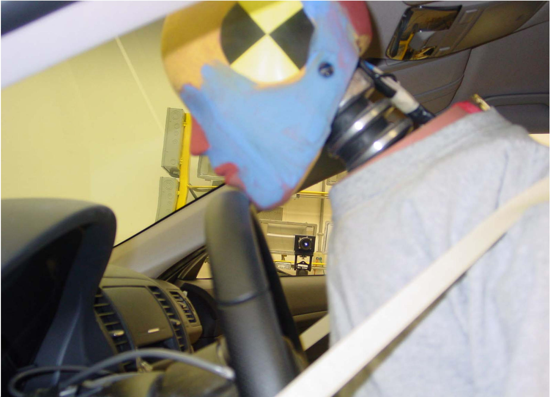
Pre-Test 5th Fem. P2 Driver Dummy Left Side Head Position View
