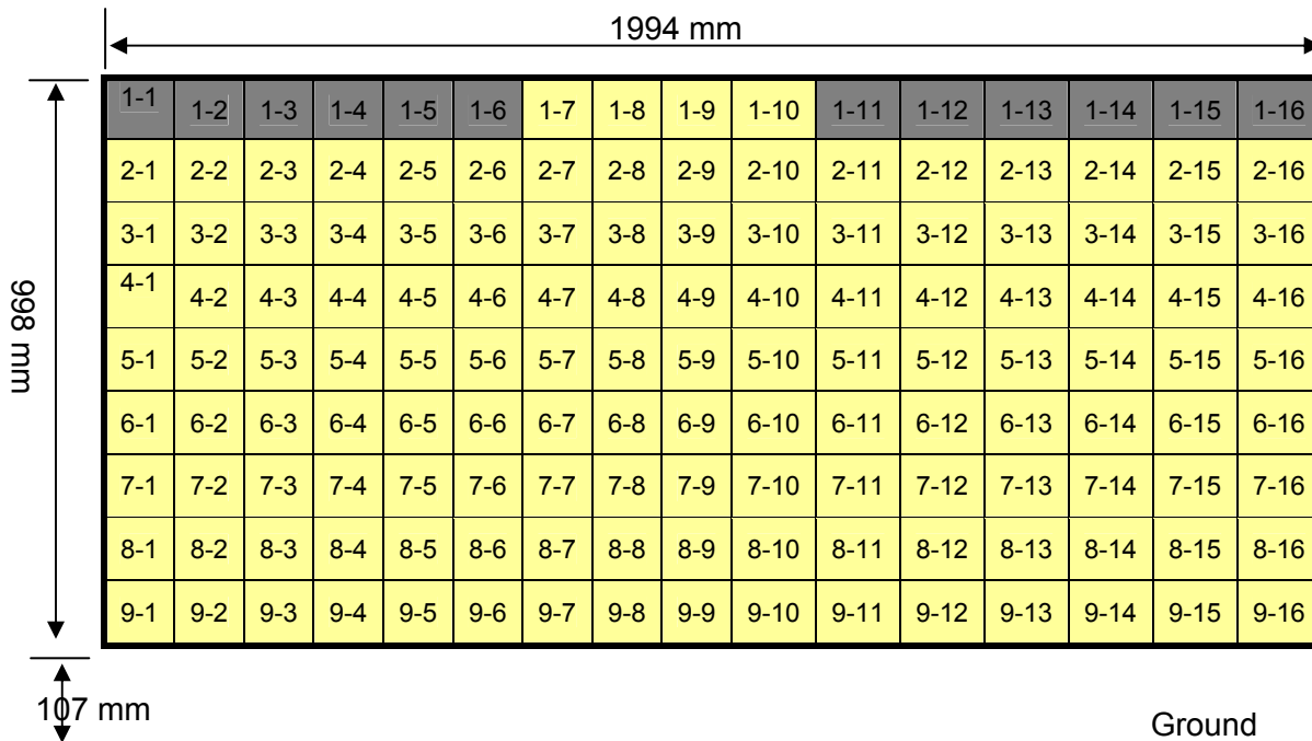
144 Load Cell Rigid Barrier Load Cell Locations on Fixed Barrier
