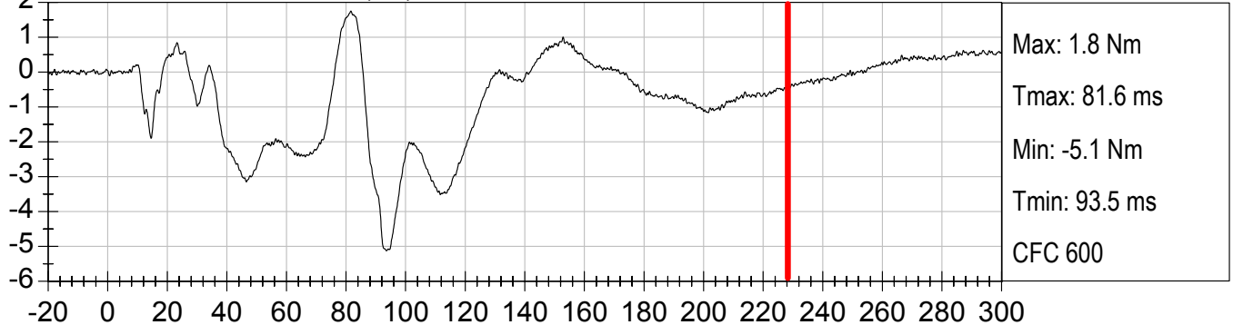
5TH FEM. DRIVER NECK MX (Nm) vs TIME (ms)
