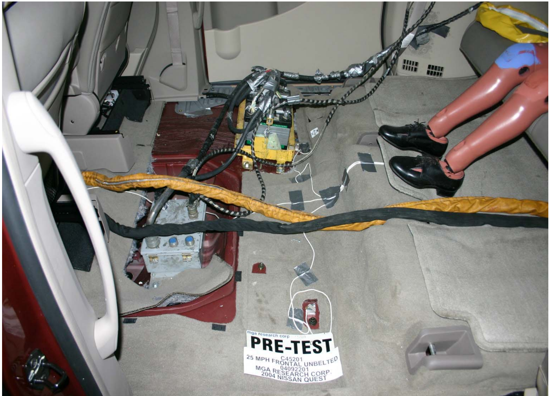
Pre-Test Center Rear Passenger Dummy Feet Position
