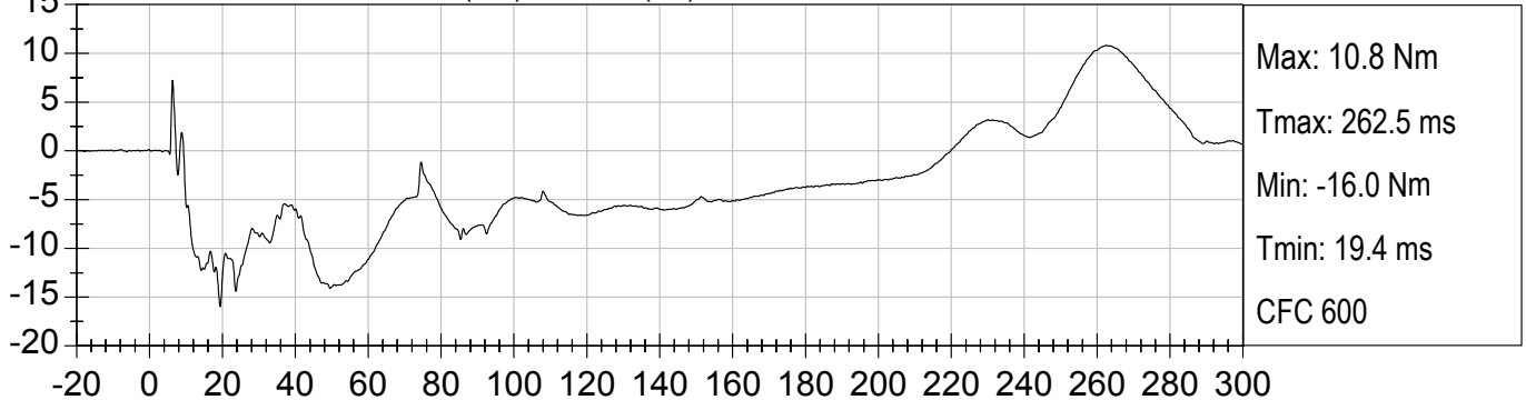
1.5 5TH FEM. DRIVER NECK MZ (Nm) vs TIME (ms)
