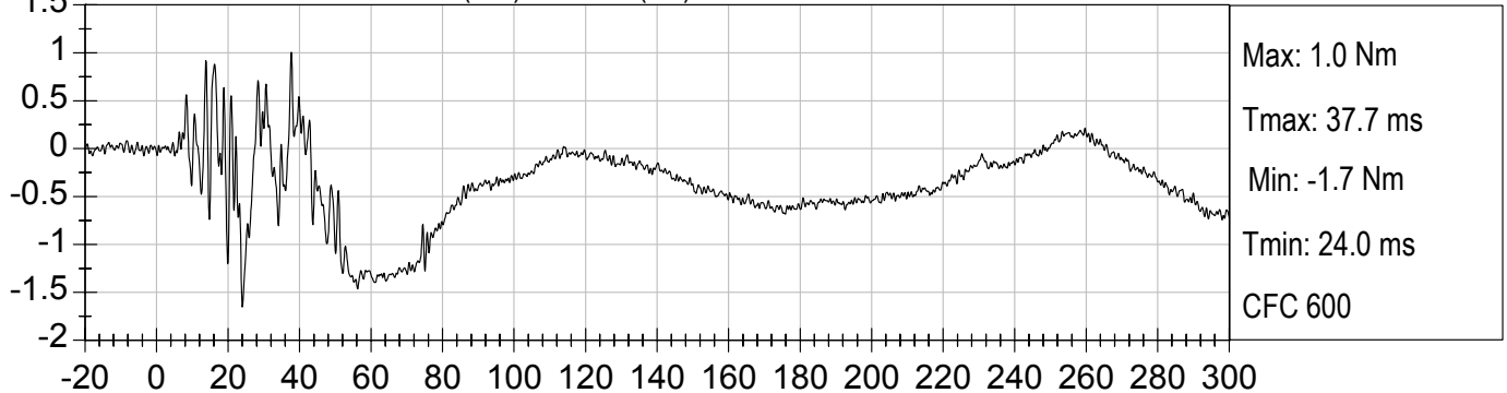
15 Drv. Occipital Condyle Moment (Nm) vs TIME (ms)
