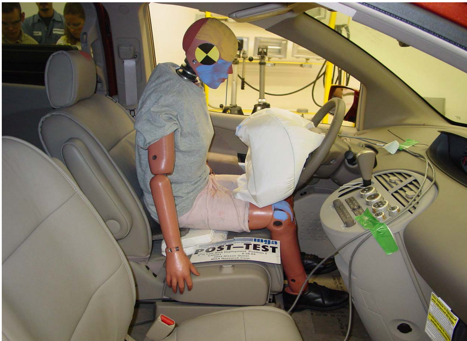
Post-Test 5th Fem. P2 Driver Dummy Right Side View (Door Open)
