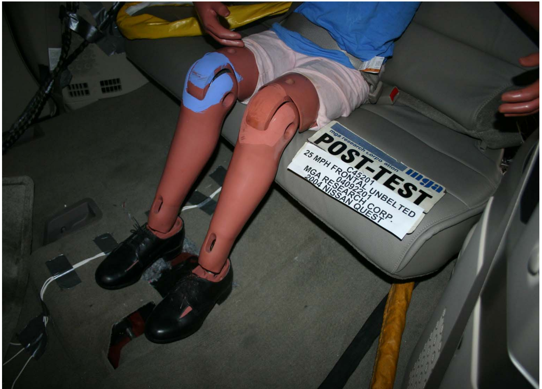
Post-Test Center Rear Passenger Dummy Feet Position
