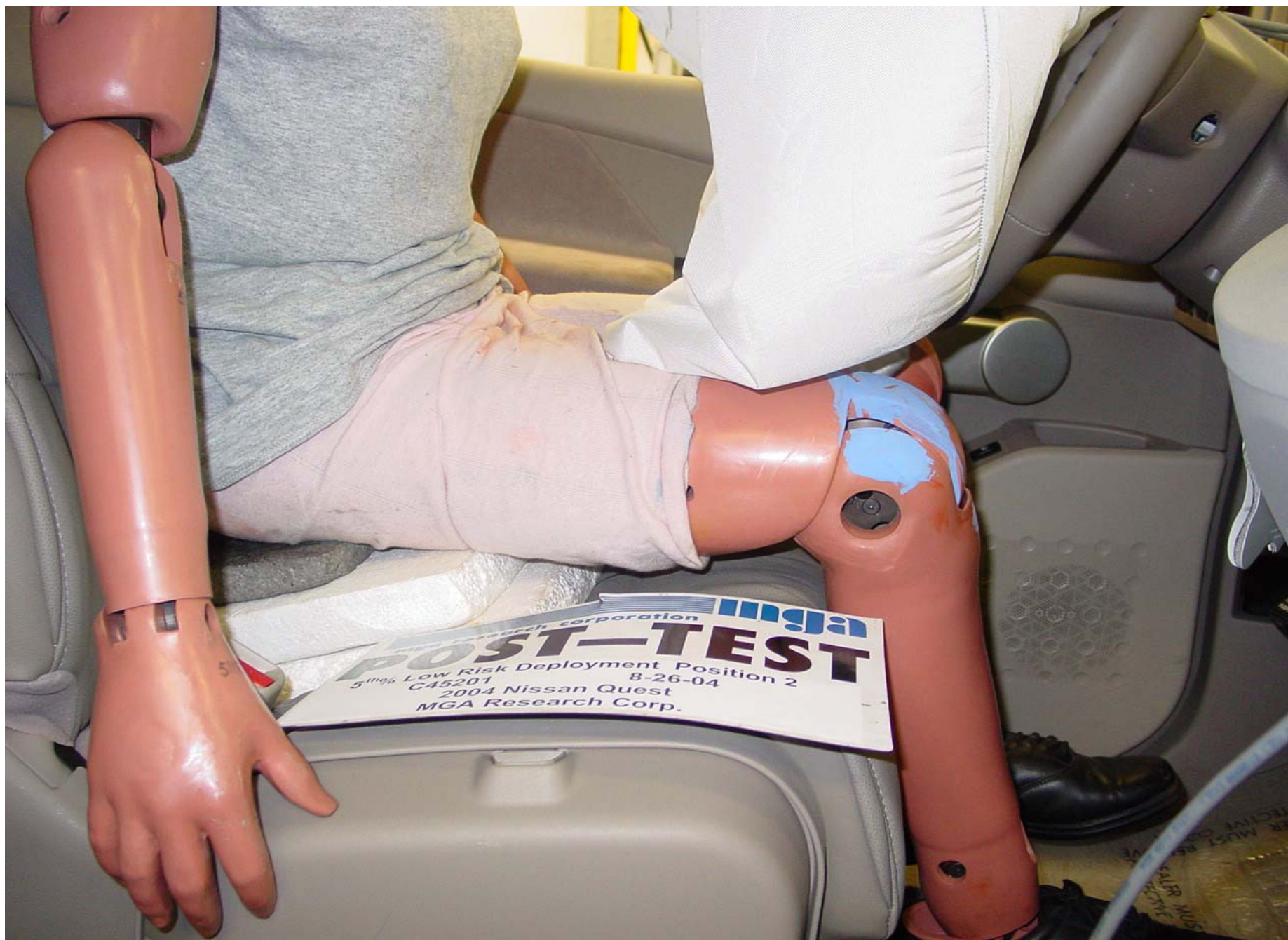
Post-Test 5th Fem. P2 Driver Dummy Right Side Knee Position View
