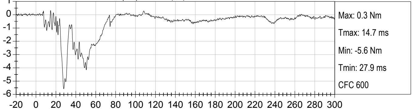
15 5TH FEM. DRIVER NECK MY (Nm) vs TIME (ms)
