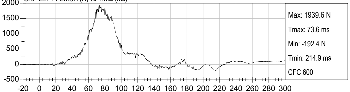
CRP SHOULDER BELT (N) vs TIME (ms)
