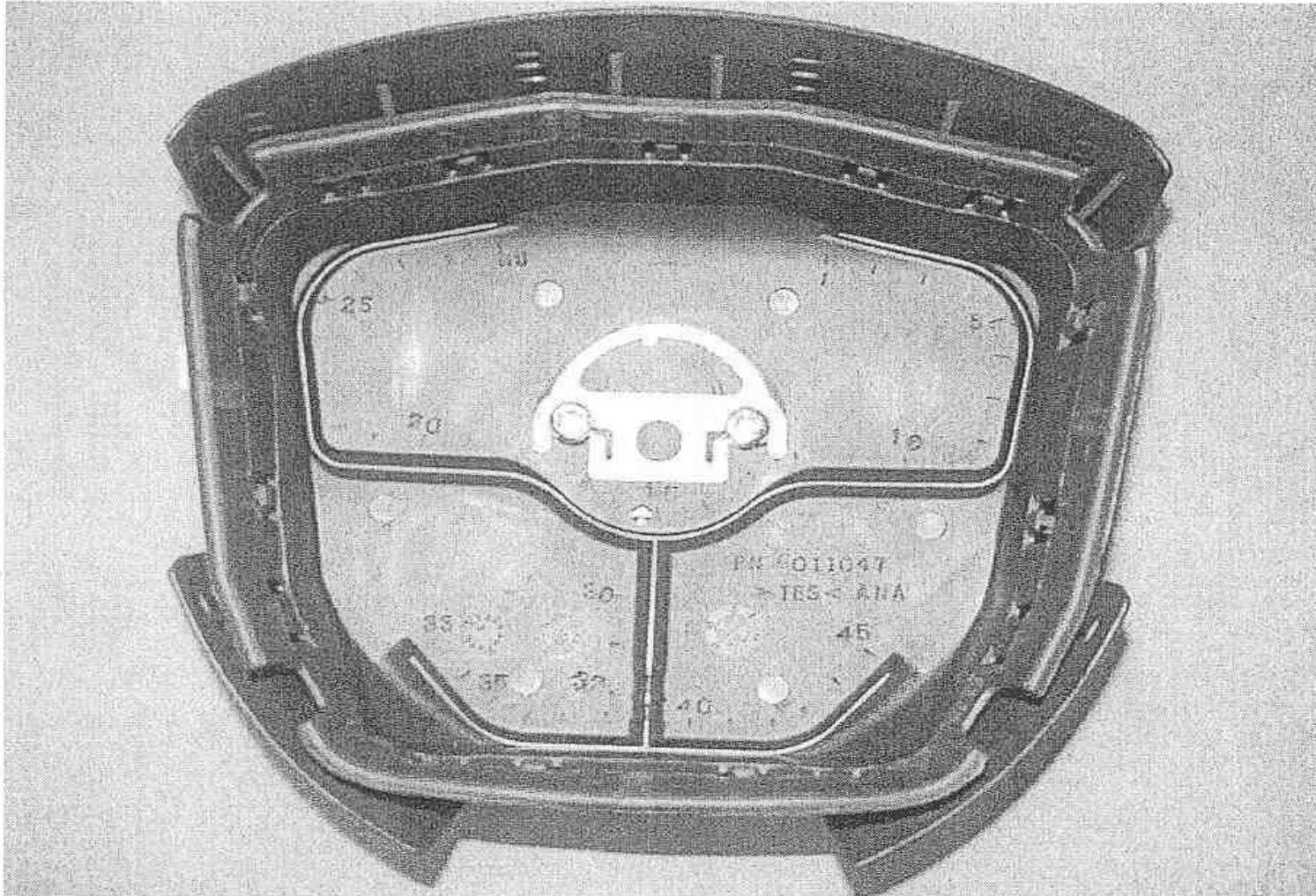
Driver side air bag cover showing “geometric center of the opening through which the air bag deploys into the occupant compartment”
