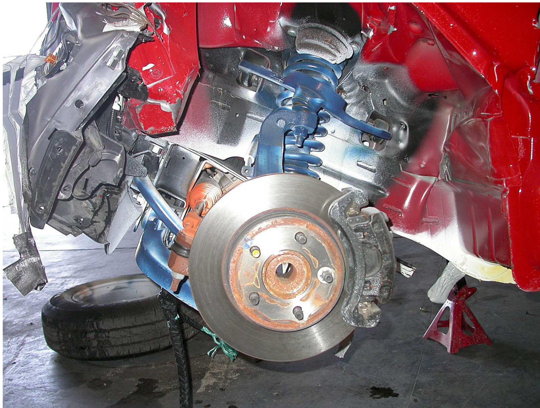
Figure A-43: Post-Test Left Front Wheel Well with Tire and Wheel Removed (Front of Test Vehicle is to the Left)
