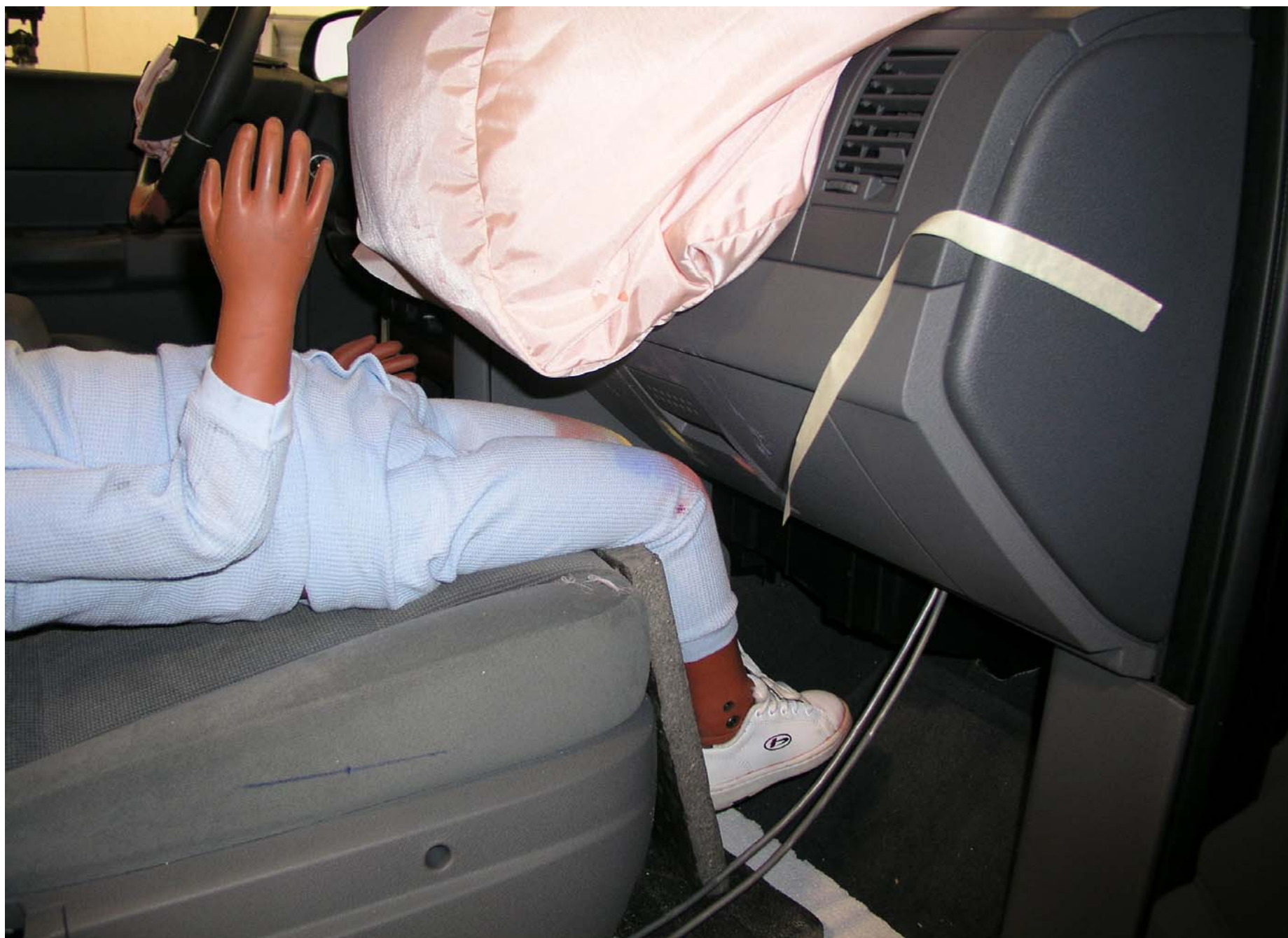
Post-Test 3YO P2 Passenger Dummy Right Knee Contact View
