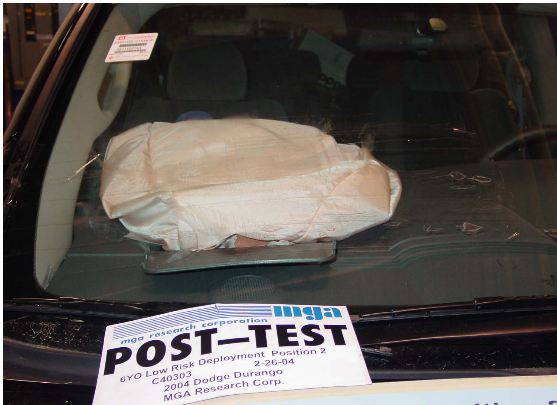
Post-Test 6YO P2 Passenger Dummy Head Frontal Position View
