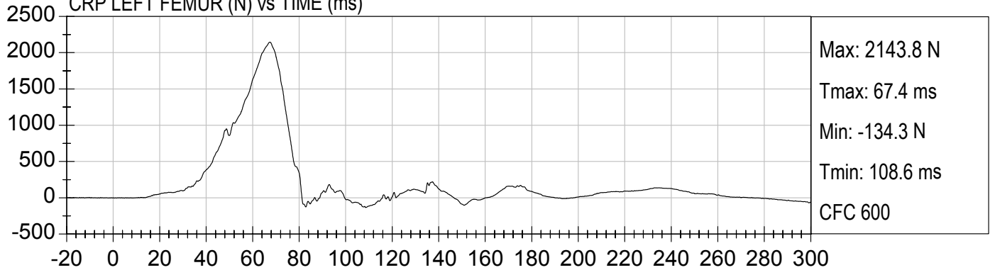
CRP LEFT FEMUR (N) vs TIME (ms)
