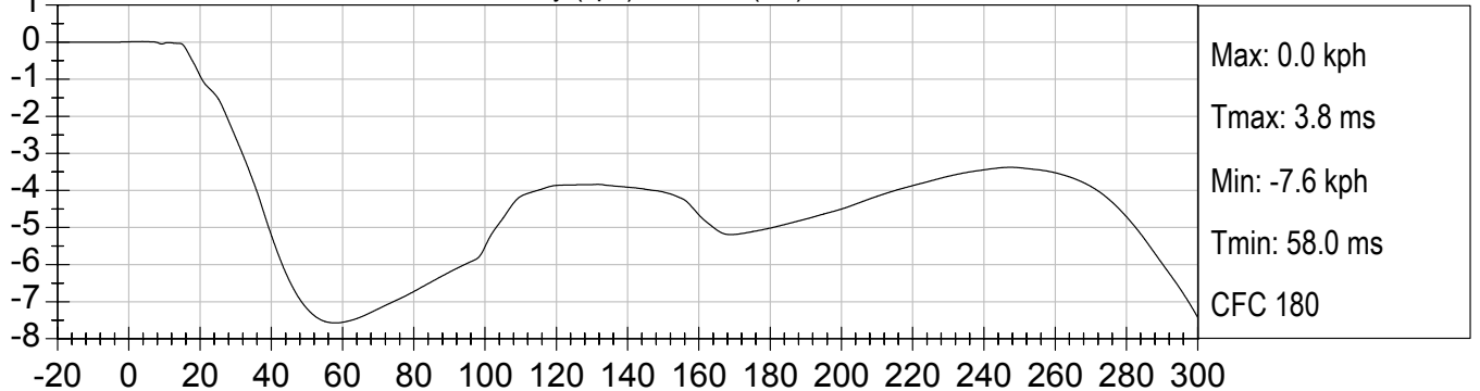
6YR OLD PASSENGER HEAD Y Velocity (kph) vs TIME (ms)
