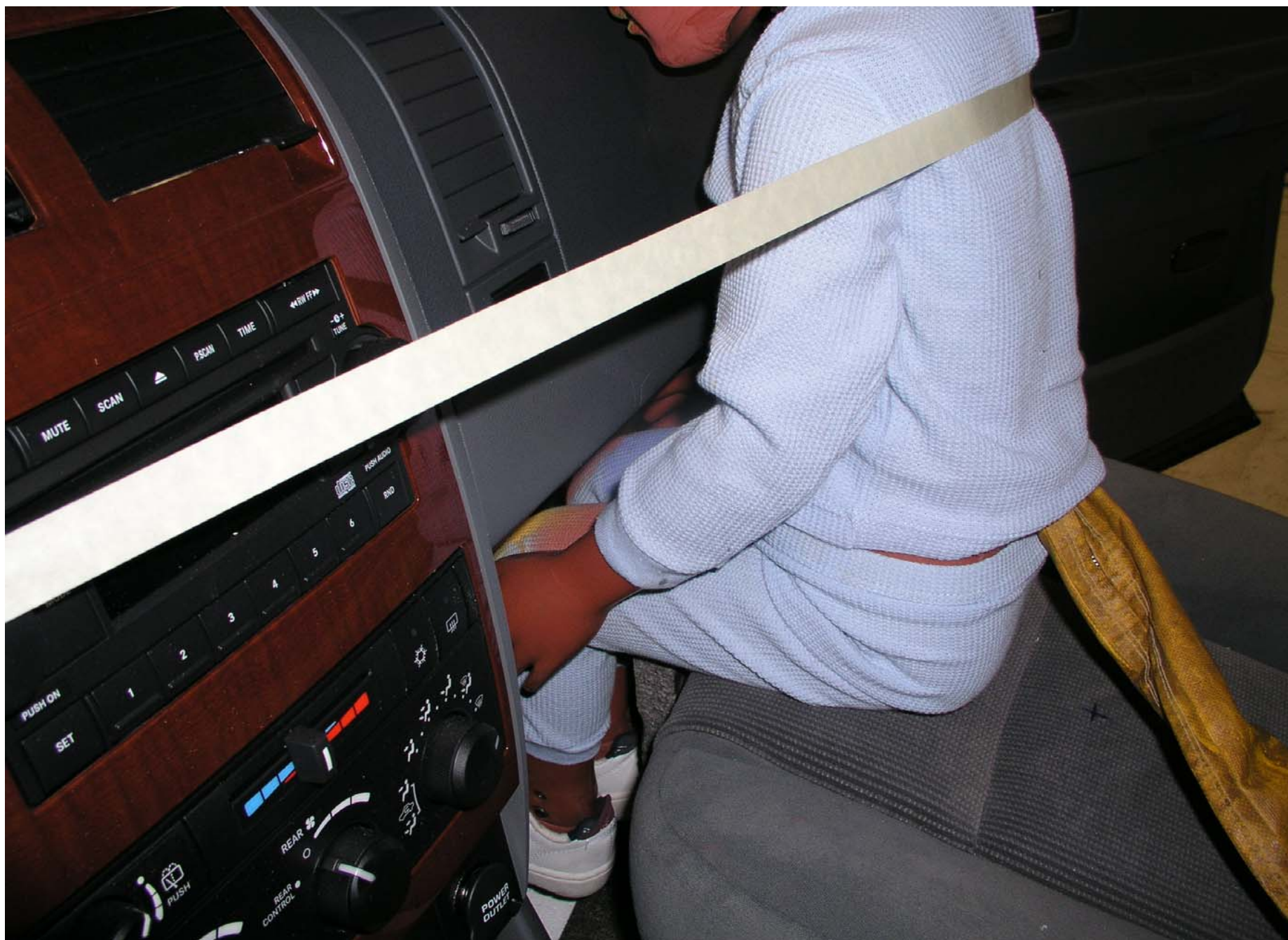
Pre-Test 3YO P2 Passenger Dummy Left Knee Position View
