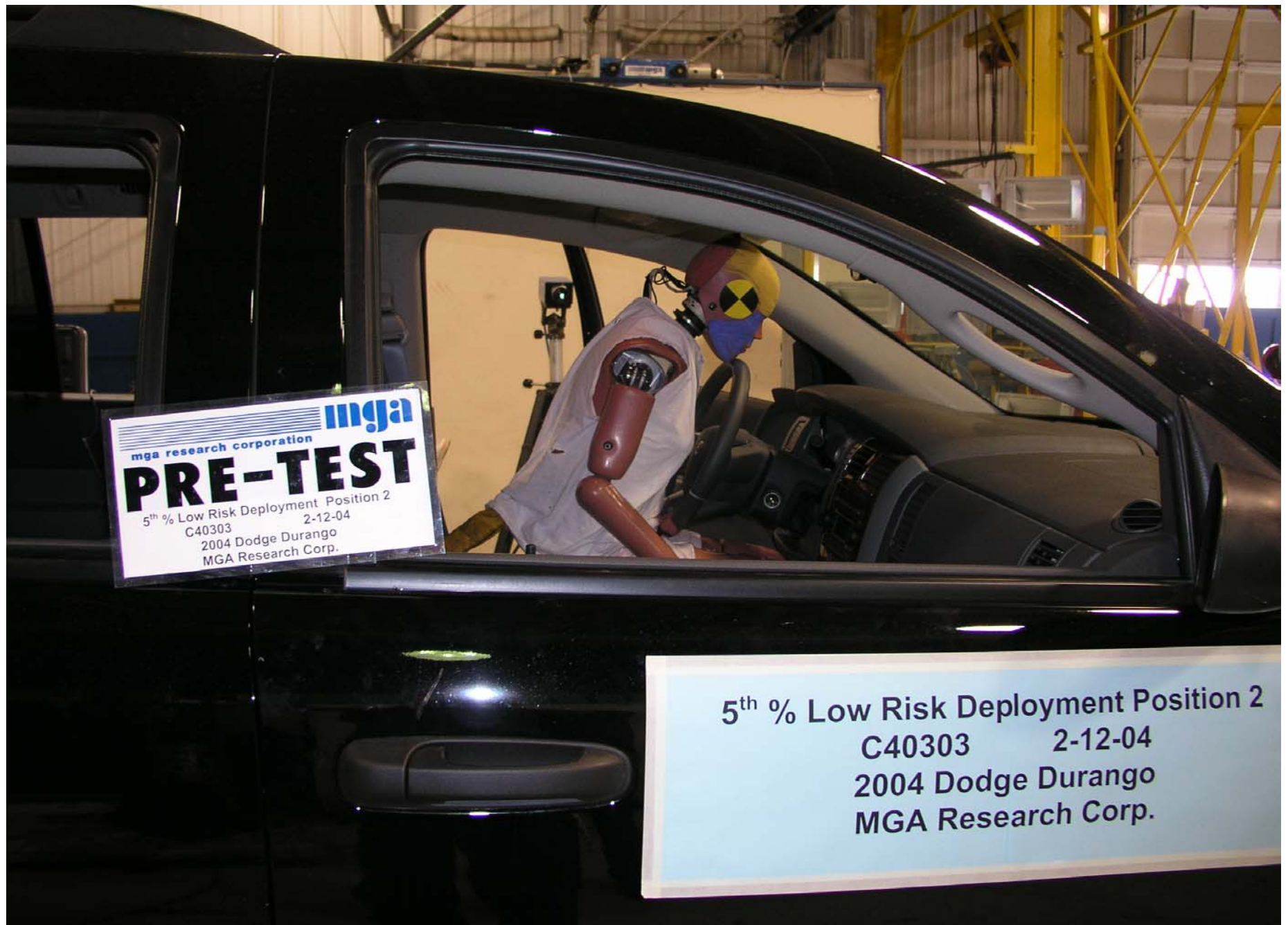
Pre-Test 5th Fem. P2 Driver Dummy Right Side View
