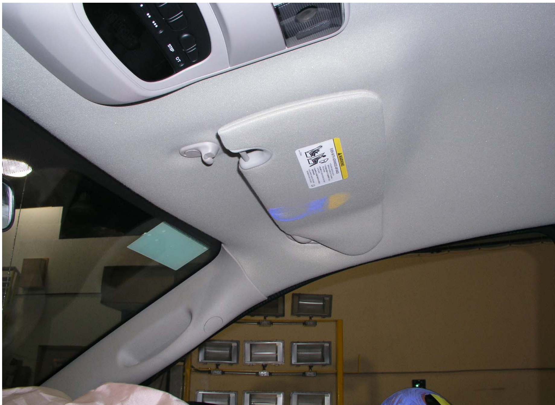
Post-Test 3YO P1 Passenger Dummy Knee Contact View (Visor)
