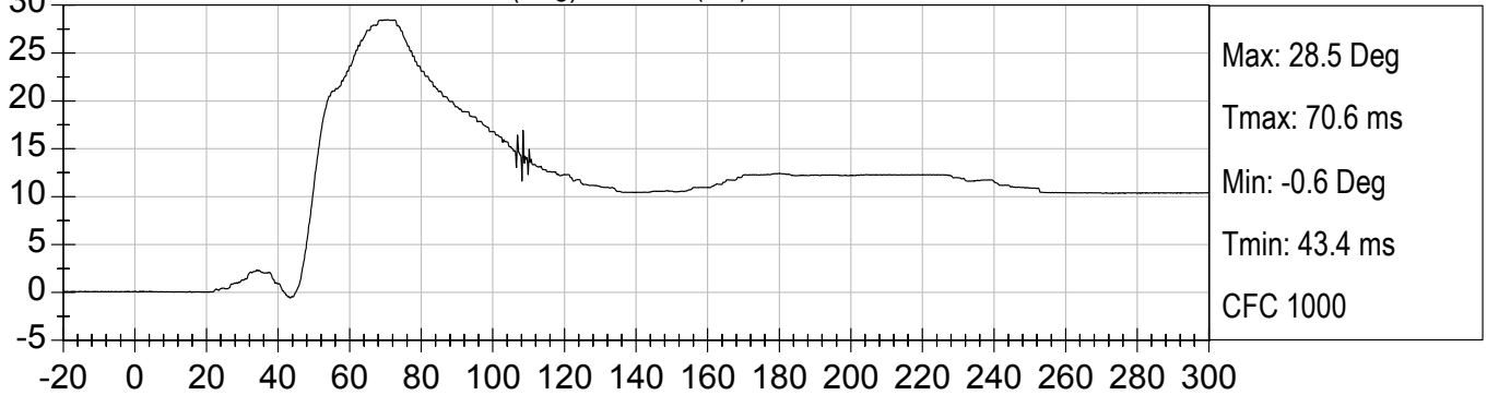
DR RT INVERSION/EVERSION (Deg) vs TIME (ms)
