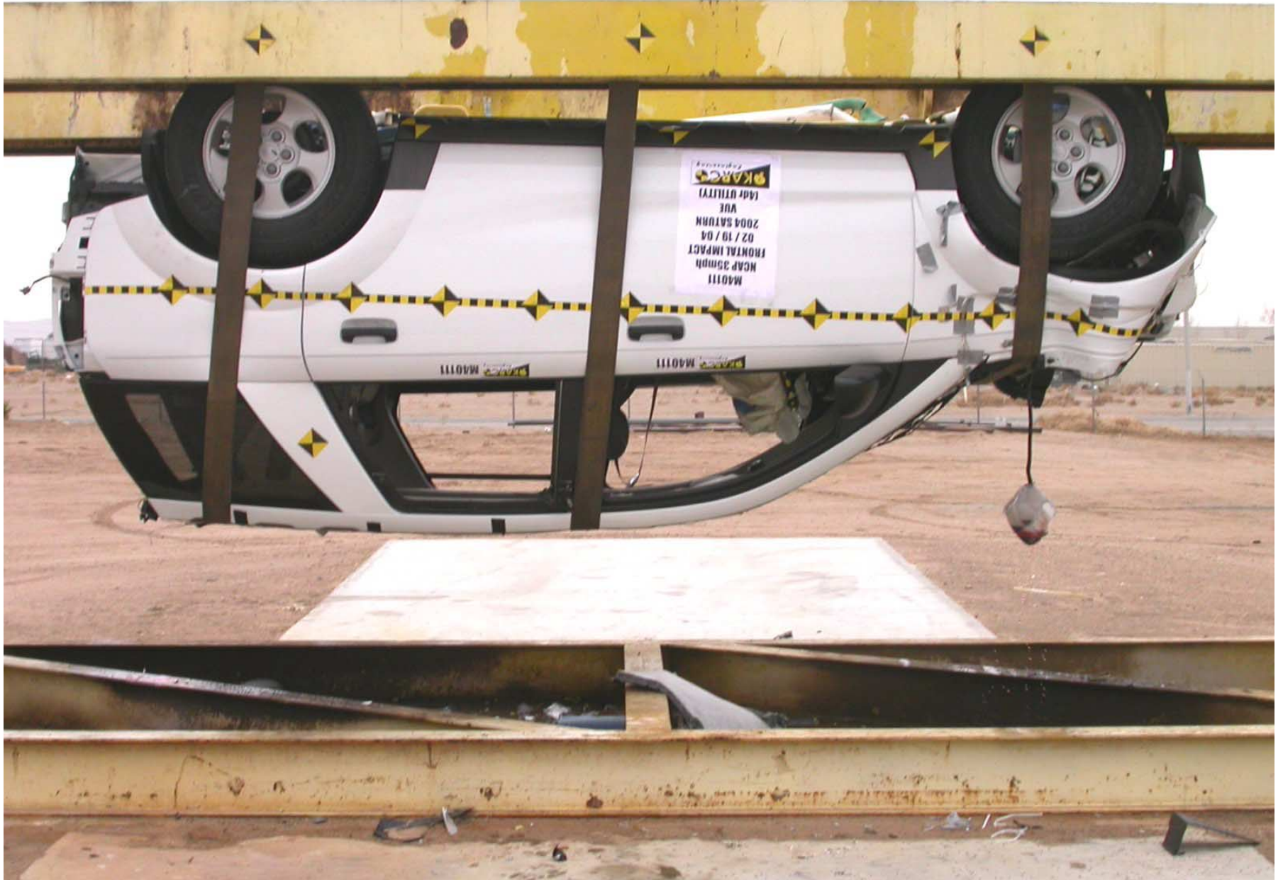
Figure A-60: Vehicle on Rollover Device
