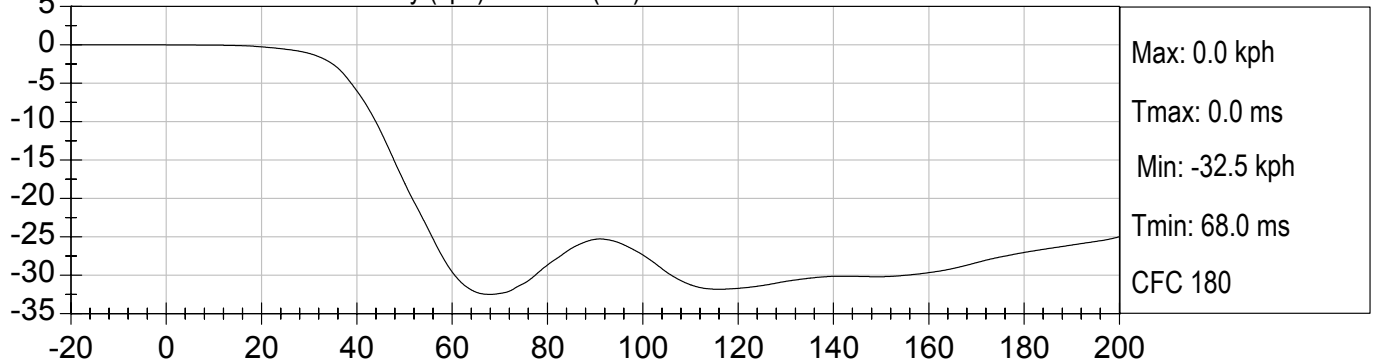
LRP CHILD CHEST Zr Velocity (kph) vs TIME (ms)
