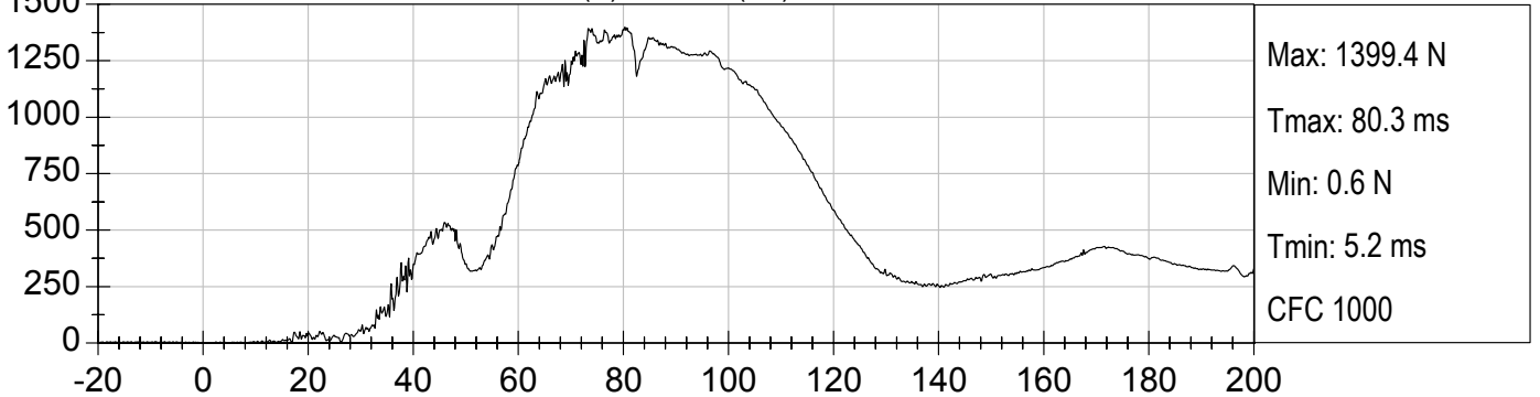
LRP CHILD UPPER NECK FResultant (N) vs TIME (ms)
