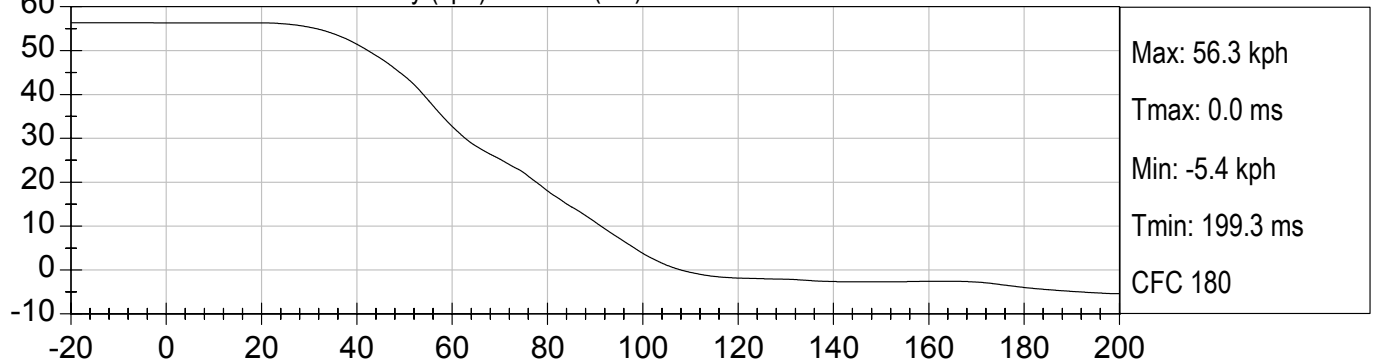
LRP CHILD CHEST Yr Velocity (kph) vs TIME (ms)
