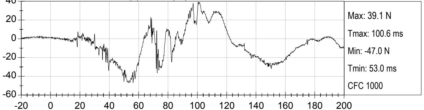
LRP CHILD UPPER NECK FZ (N) vs TIME (ms)
