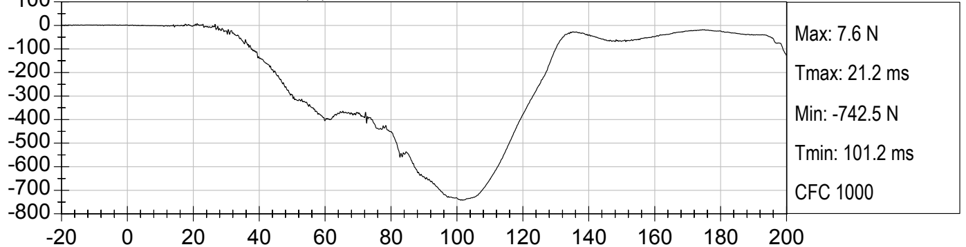
LRP CHILD UPPER NECK FY (N) vs TIME (ms)
