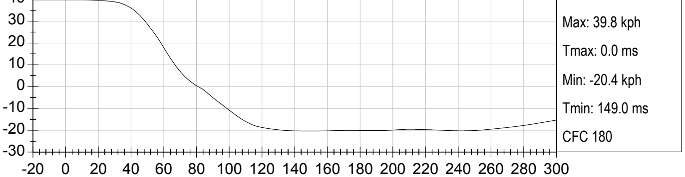
CRP CHEST X Velocity (kph) vs TIME (ms)
