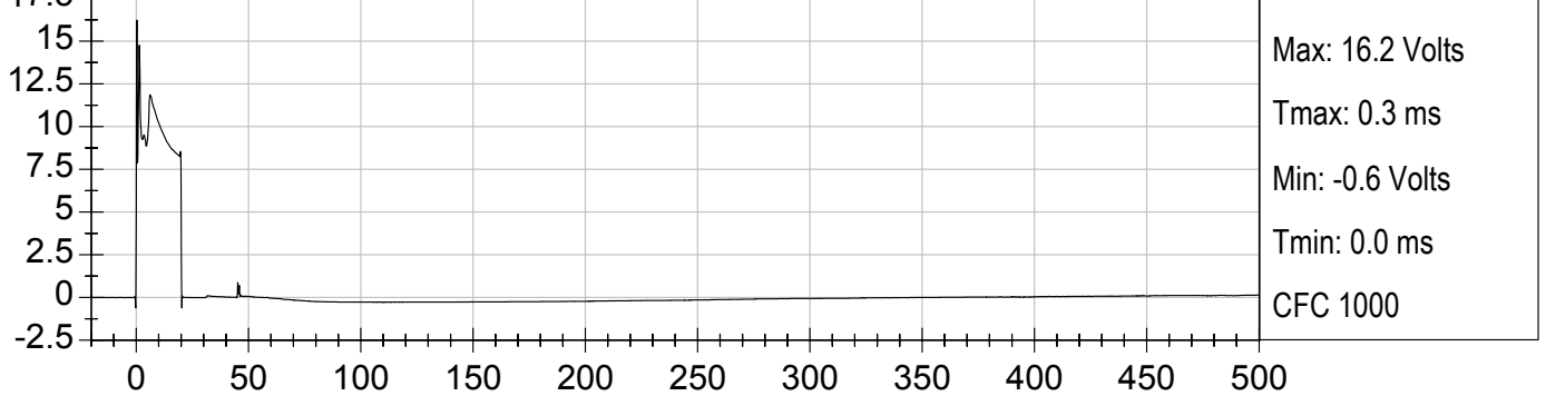
FIRE VOLTAGE #1 (Volts) vs TIME (ms)
