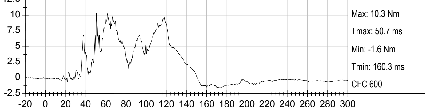
DRIVER NECK MX (Nm) vs TIME (ms)
