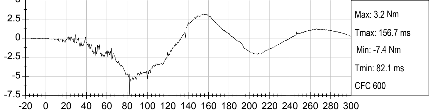
DRIVER NECK MZ (Nm) vs TIME (ms)
