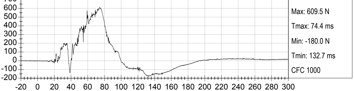
DRIVER NECK FX (N) vs TIME (ms)
