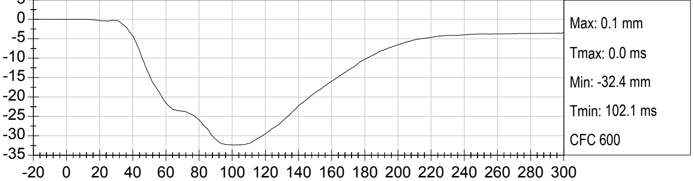
CRP CHEST DISPLACEMENT (mm) vs TIME (ms)
