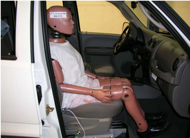
Unbelted 5th Percentile Female Reactivation Seat, Rearward Seat Track
