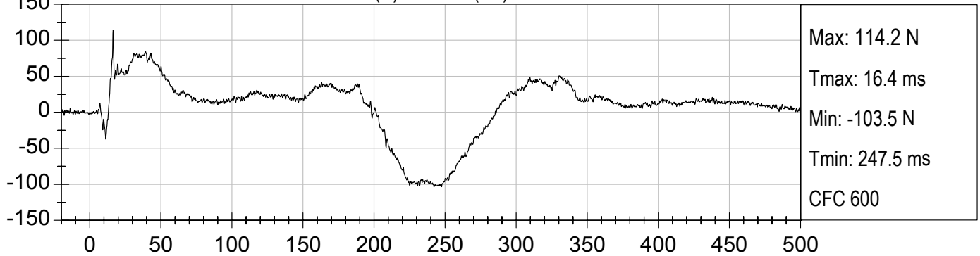
5TH FEM. P1 DRIVER RIGHT FEMUR (N) vs TIME (ms)
