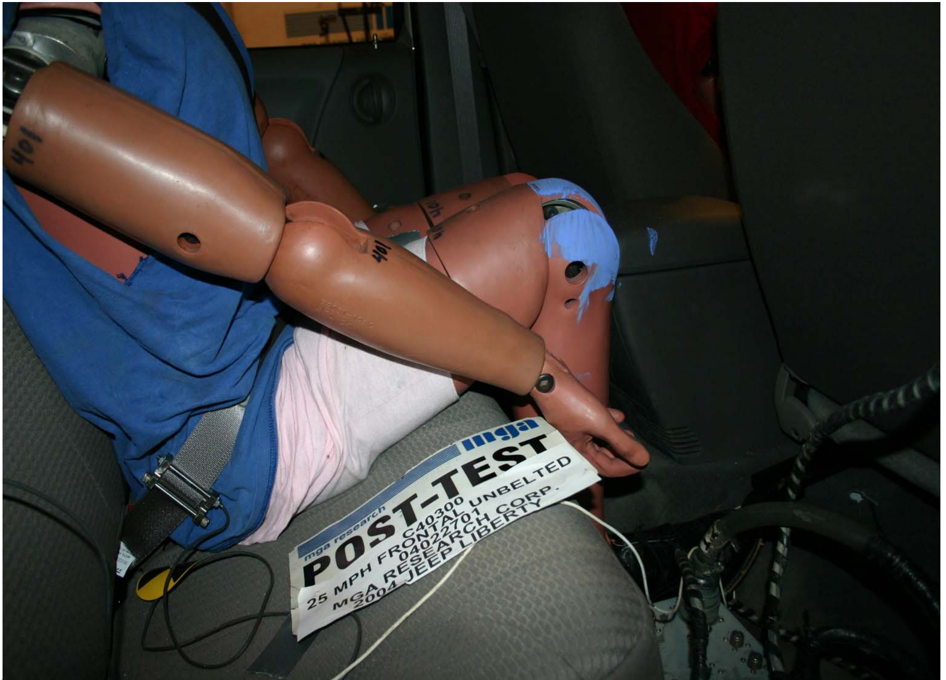
Post-Test Rear Passenger Right Side Knee Bolster View
