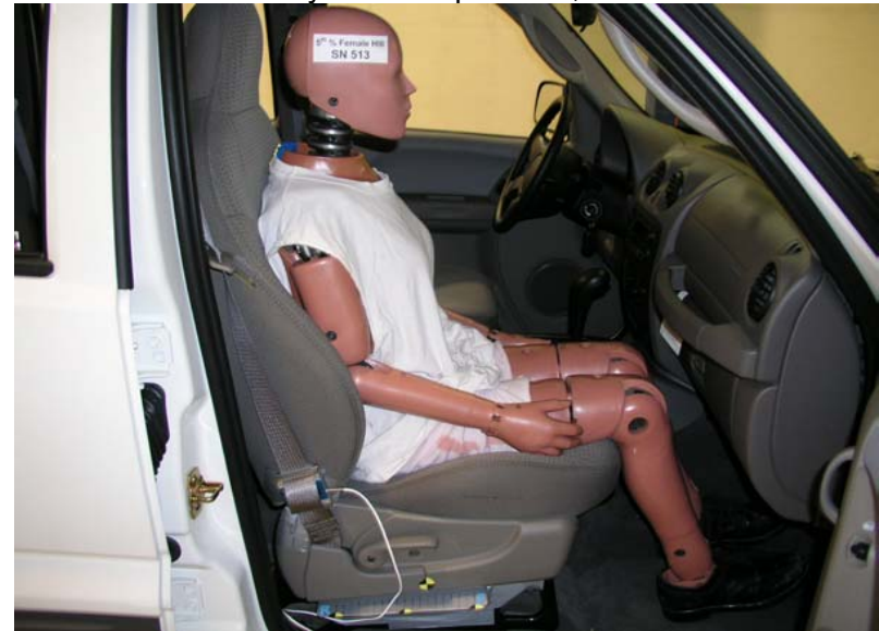
Unbelted 5th Percentile Female Reactivation Seat, Forward Seat Track
