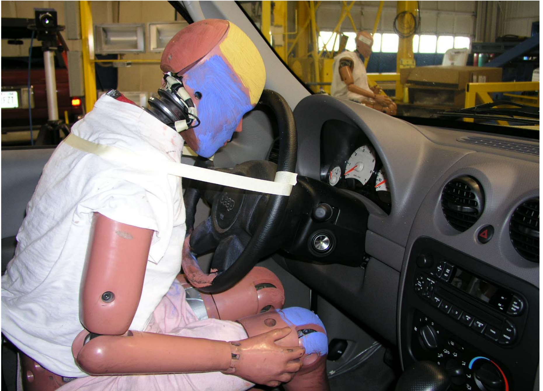
Pre-Test 5th Fem. P1 Driver Dummy Right Side View (Door Open, Closeup)
