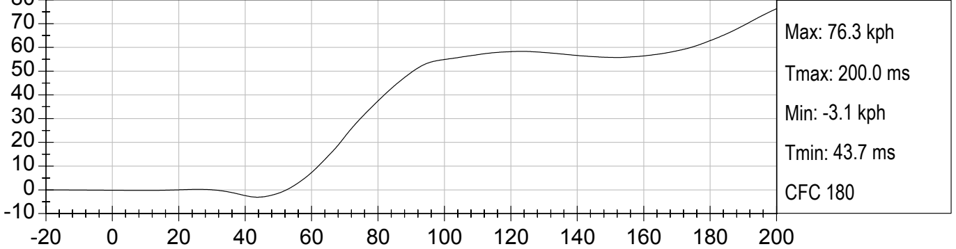
LRP CHILD HEAD Zr Velocity (kph) vs TIME (ms)
