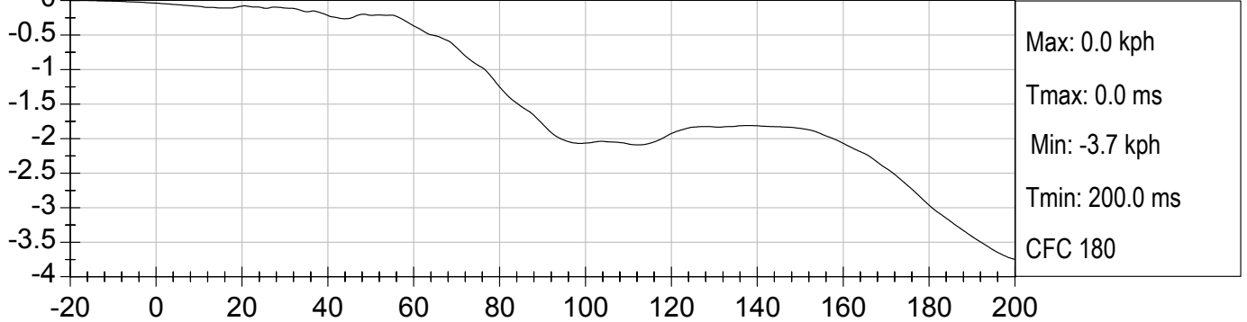
LRP CHILD HEAD Yr Velocity (kph) vs TIME (ms)
