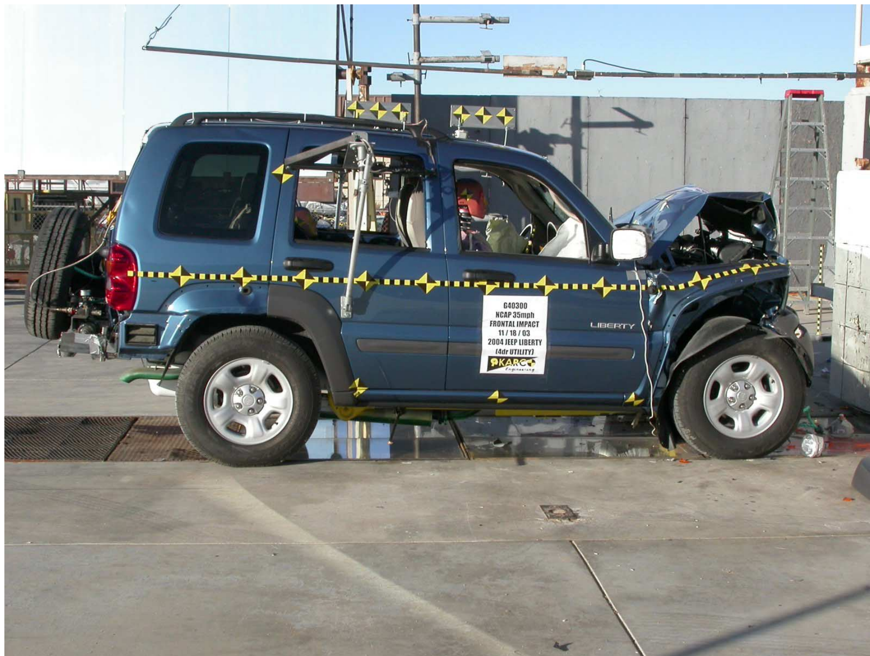
Figure A-11: Post-Test Right Side View (Correct NHTSA # is M40300)
