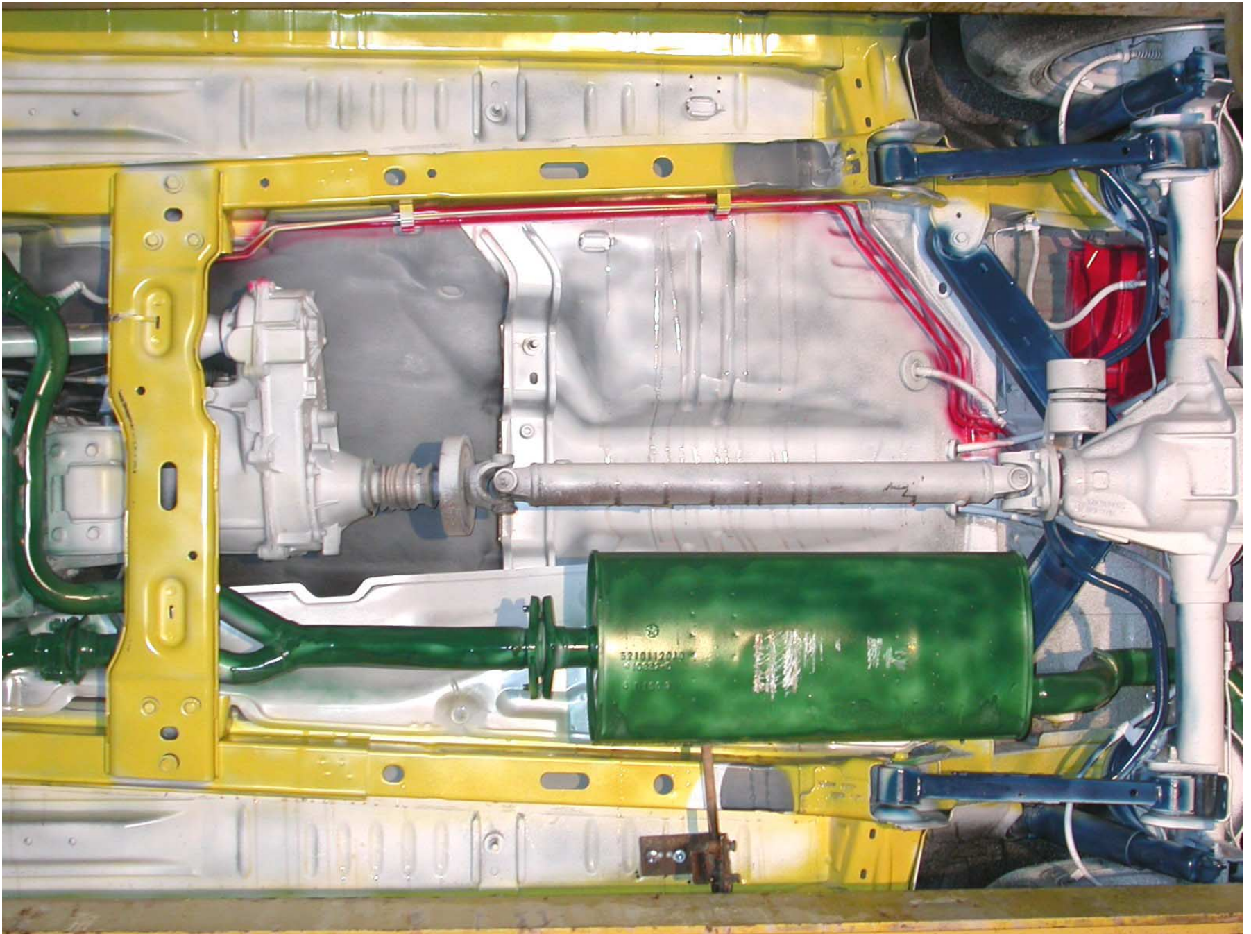
Figure A-27: Post-Test Mid Underbody View (Correct NHTSA # is M40300)
