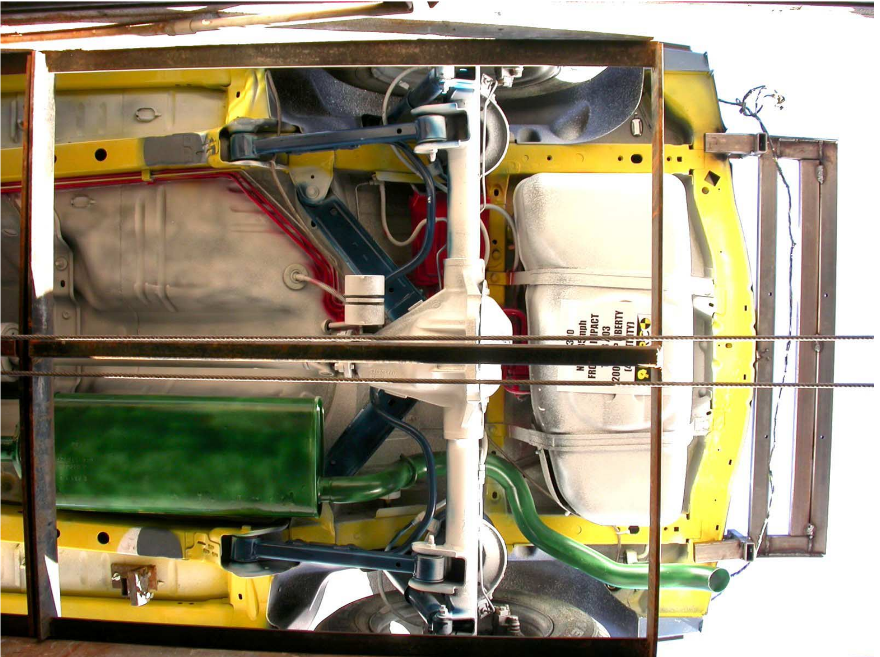
Figure A-28: Pre-Test Rear Underbody View (Correct NHTSA # is M40300)
