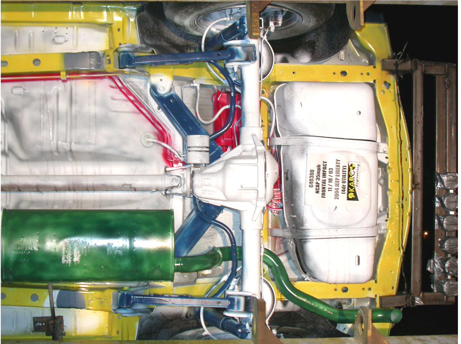
Figure A-29: Post-Test Rear Underbody View (Correct NHTSA # is M40300)
