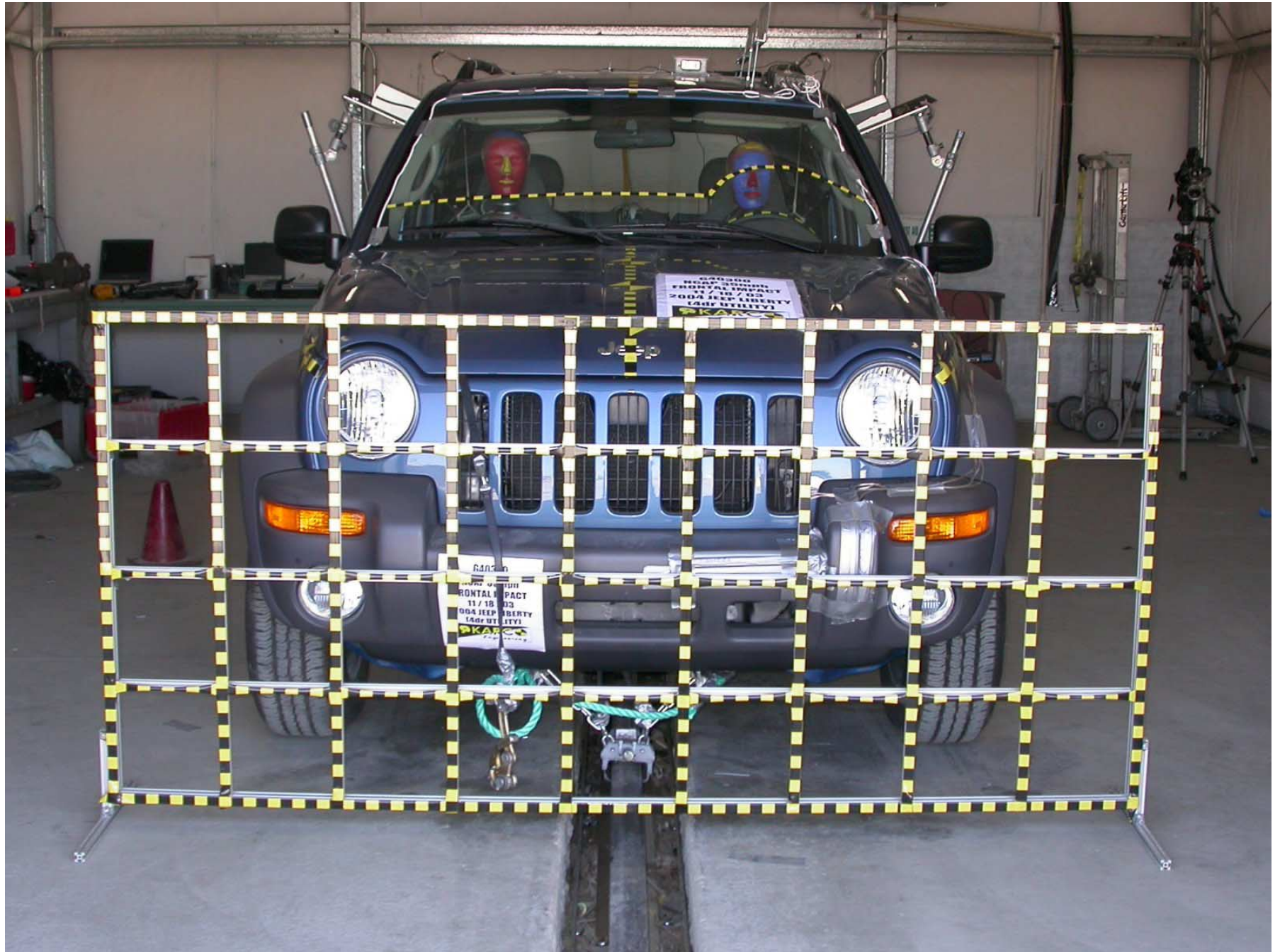
Figure A-1: Load Cell Location (Correct NHTSA # is M40300)
