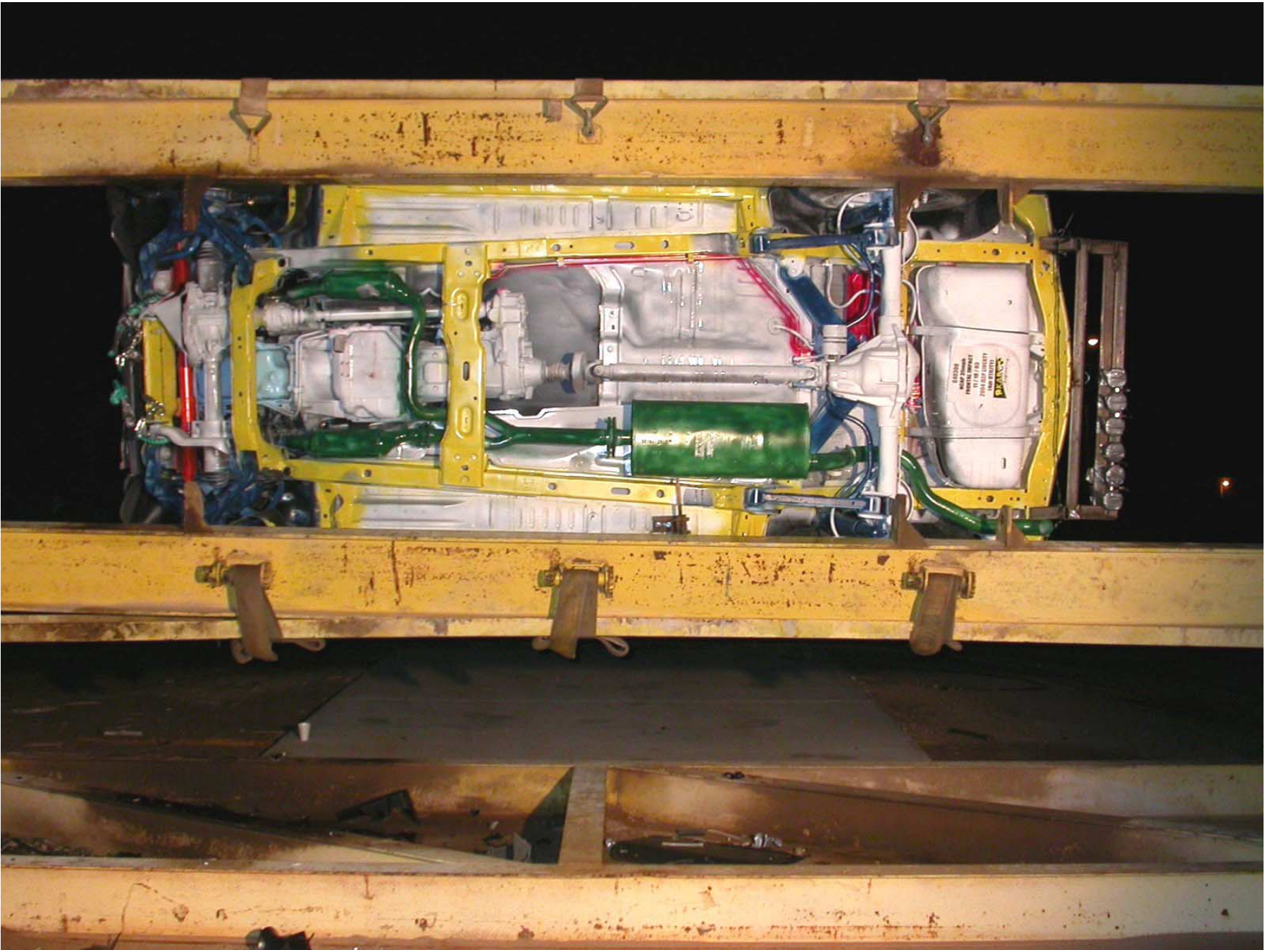
Figure A-61: Vehicle on Rollover Device (Correct NHTSA # is M40300)
