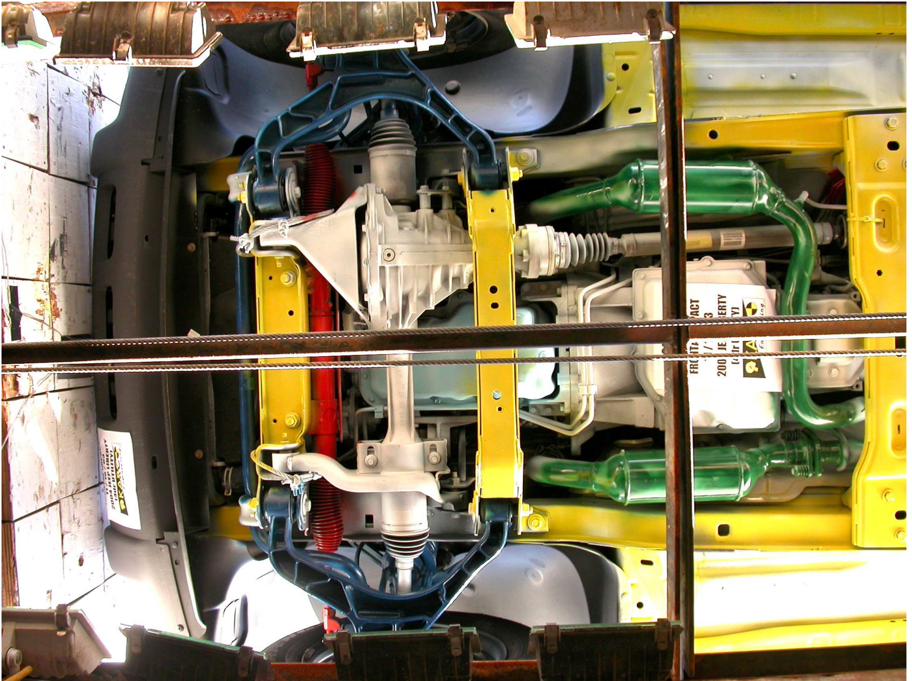
Figure A-24: Pre-Test Front Underbody View (Correct NHTSA # is M40300)
