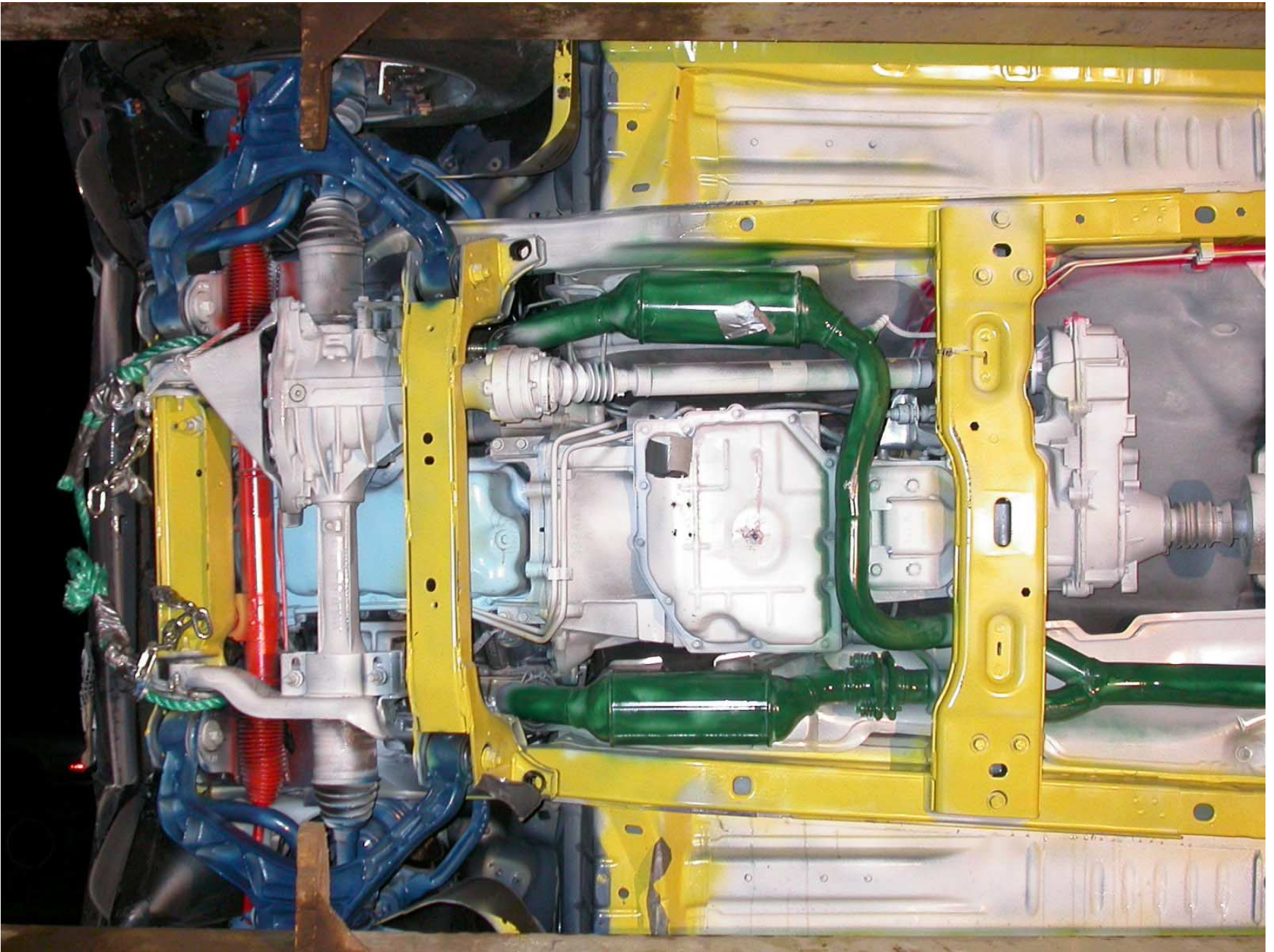
Figure A-25: Post-Test Front Underbody View (Correct NHTSA # is M40300)
