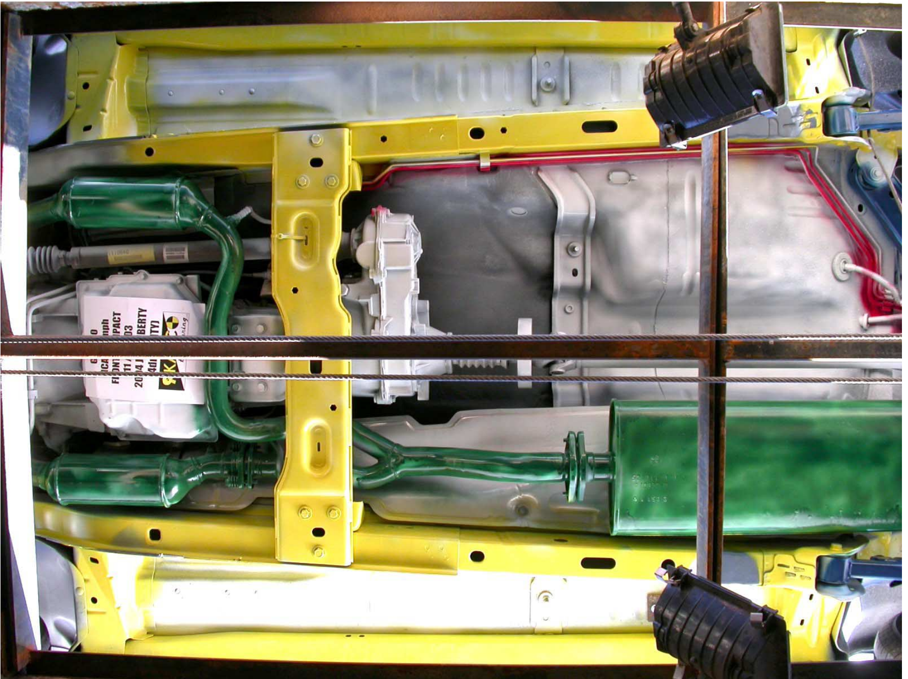
Figure A-26: Pre-Test Mid Underbody View (Correct NHTSA # is M40300)
