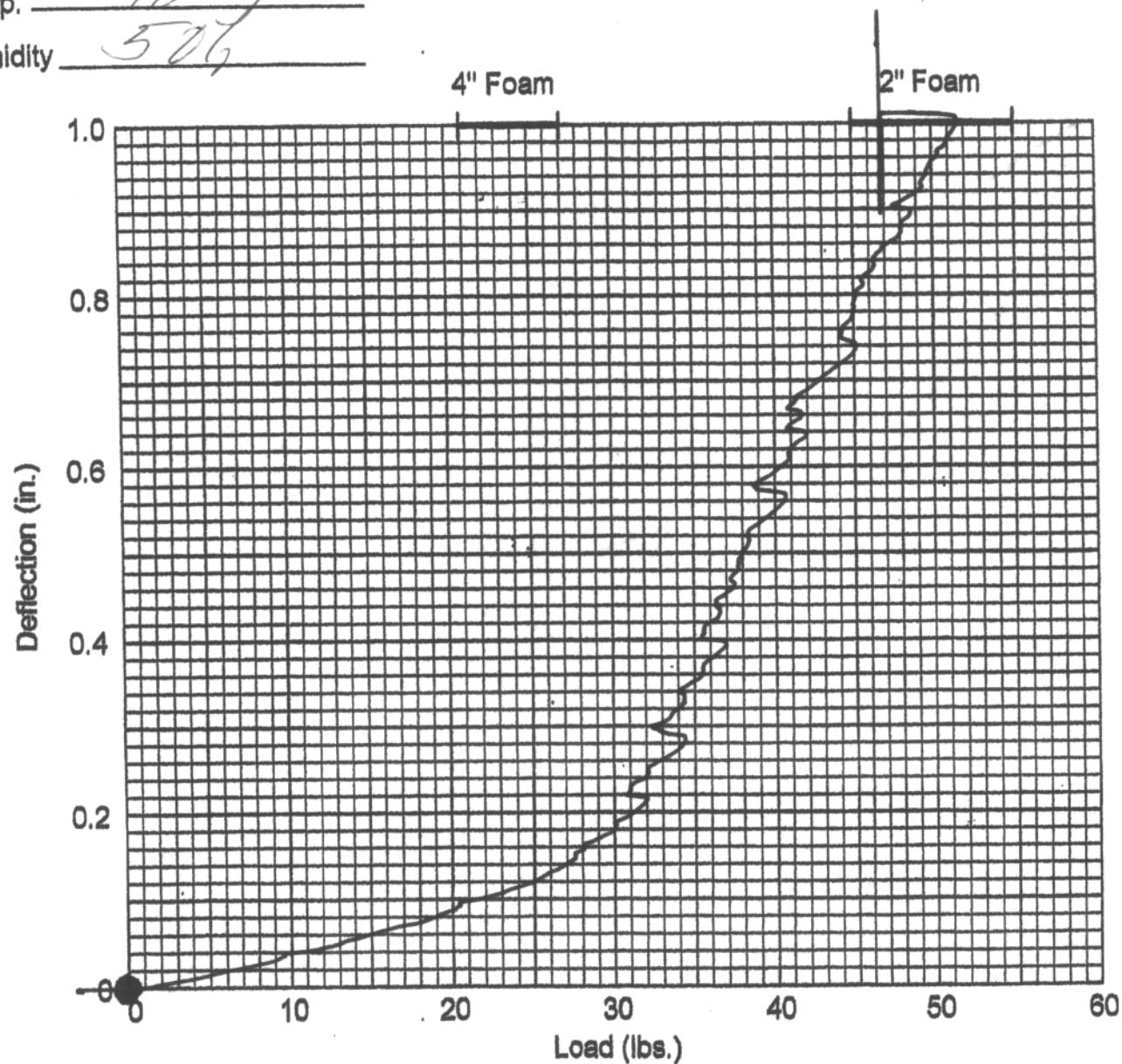
Compression - Deflection Resistance Test Child Seat Foam
