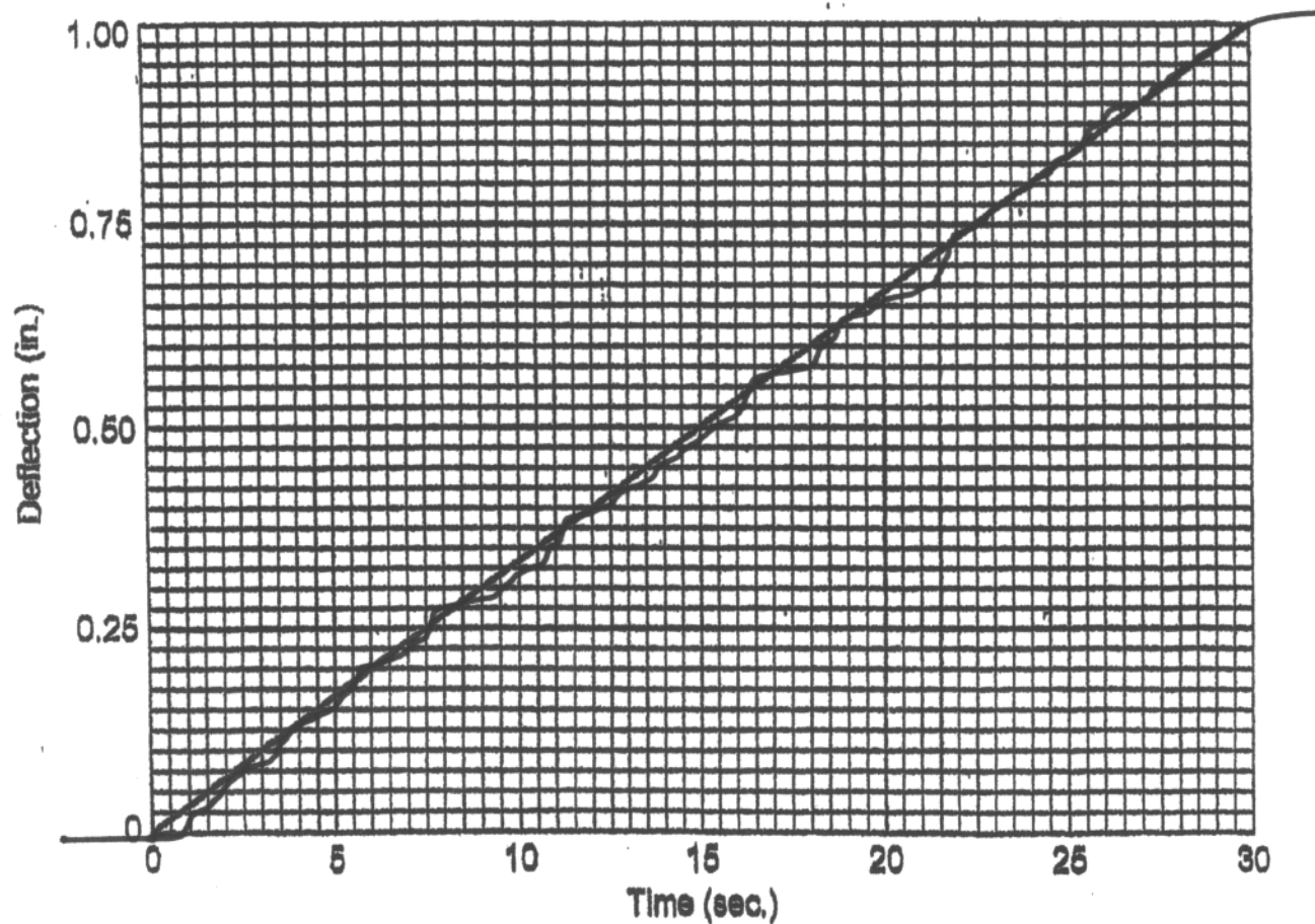
Compression - Deflection Resistance Test Child Seat Foam
