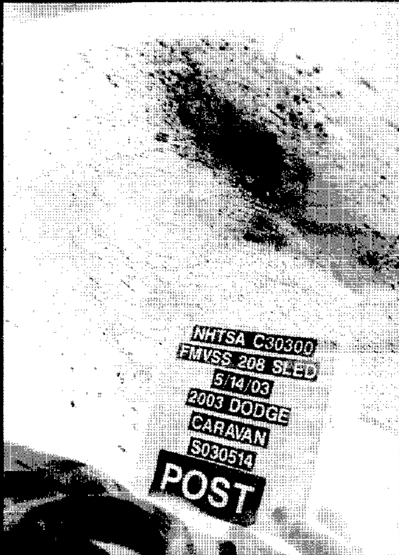
Figure A-26. Post-Test Passenger Head Contact – View 1
