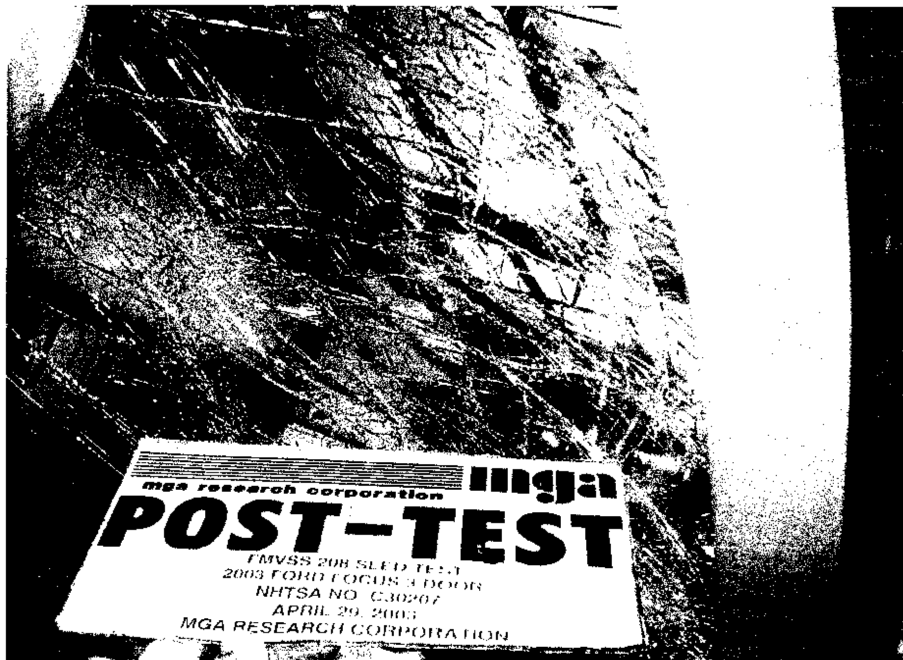
Post-Test Passenger Dummy Head Contact View (windshield)
