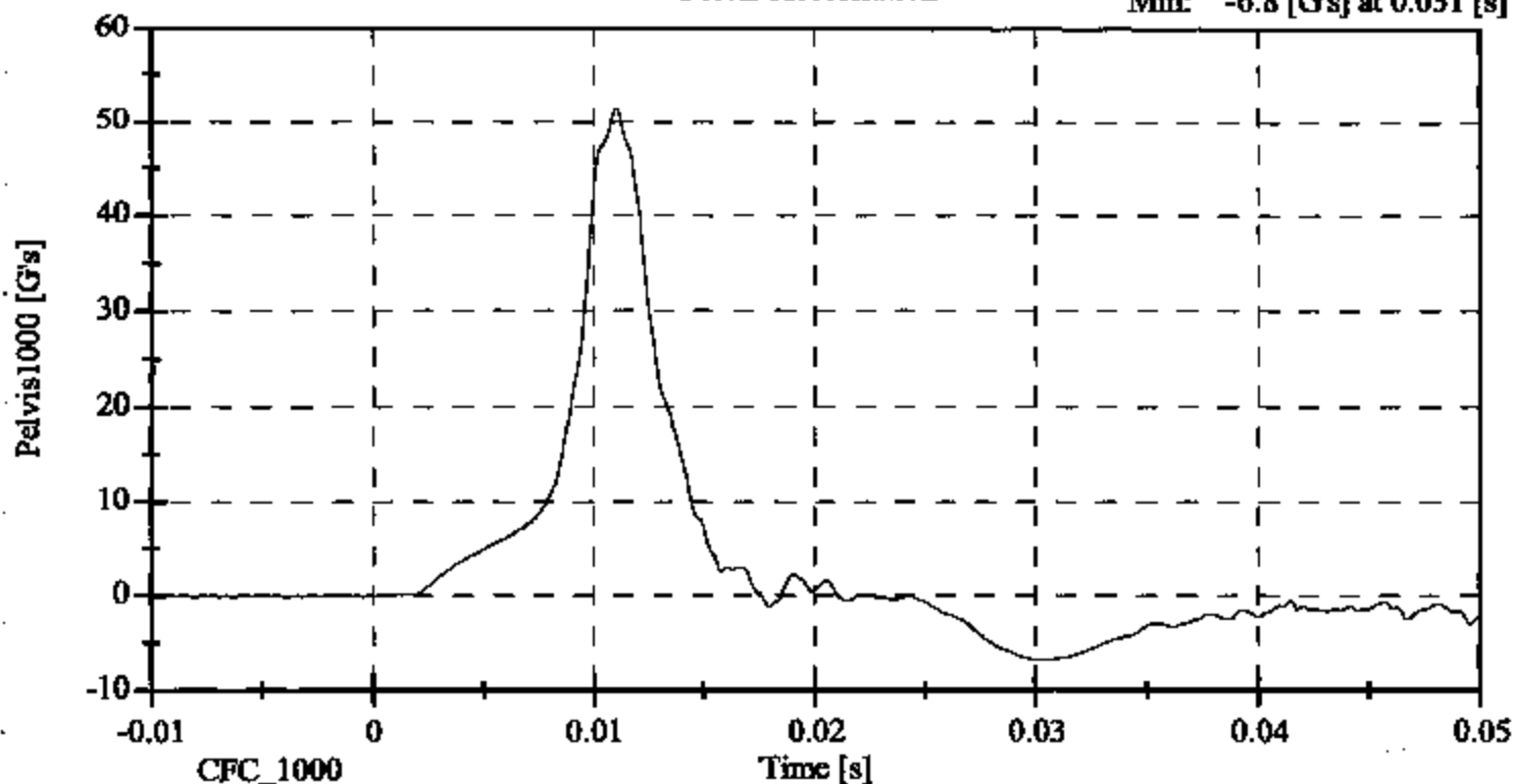
Pelvis Acceleration
