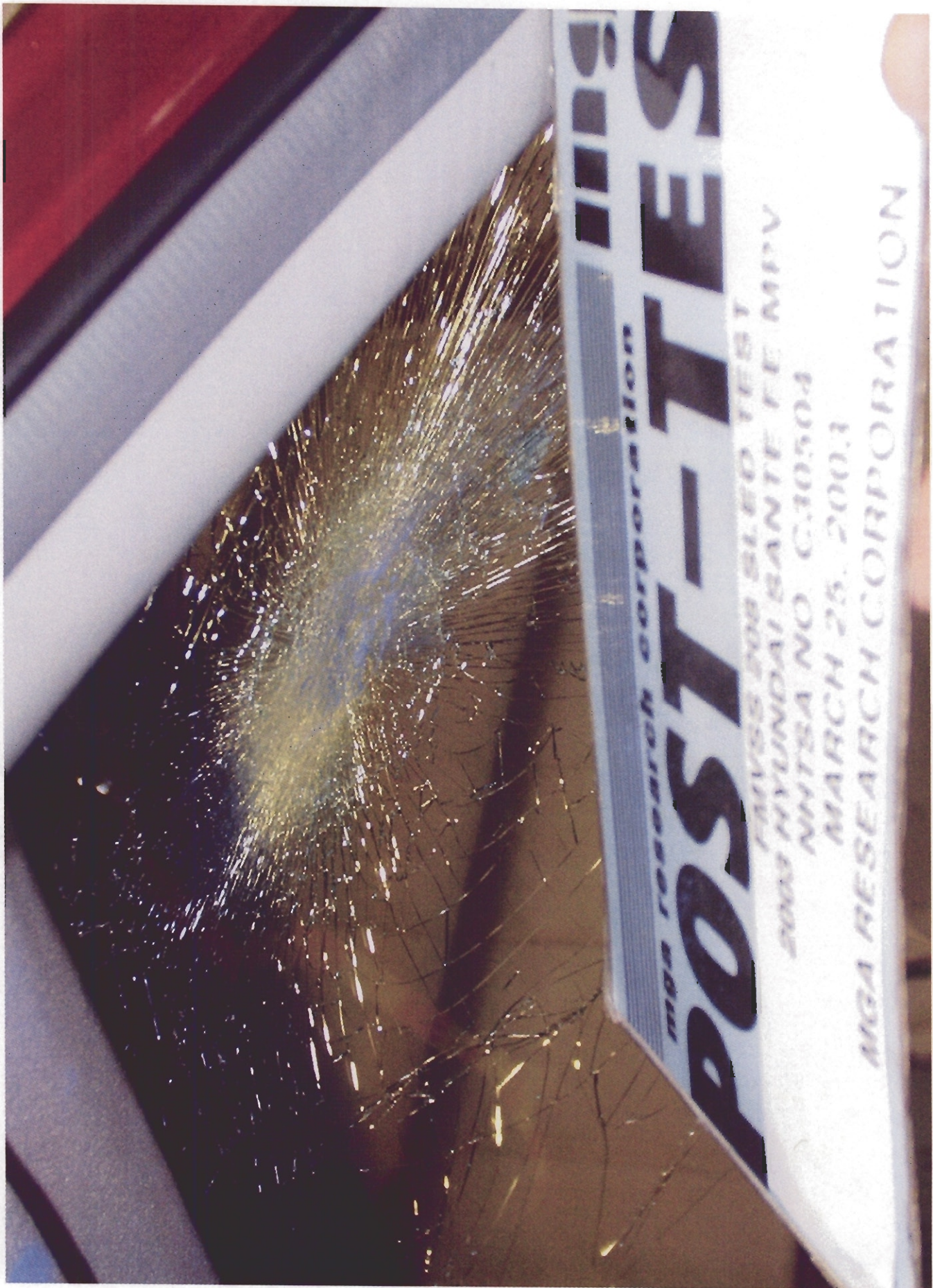
Post-Test Passenger Dummy Head Contact (windshield)
