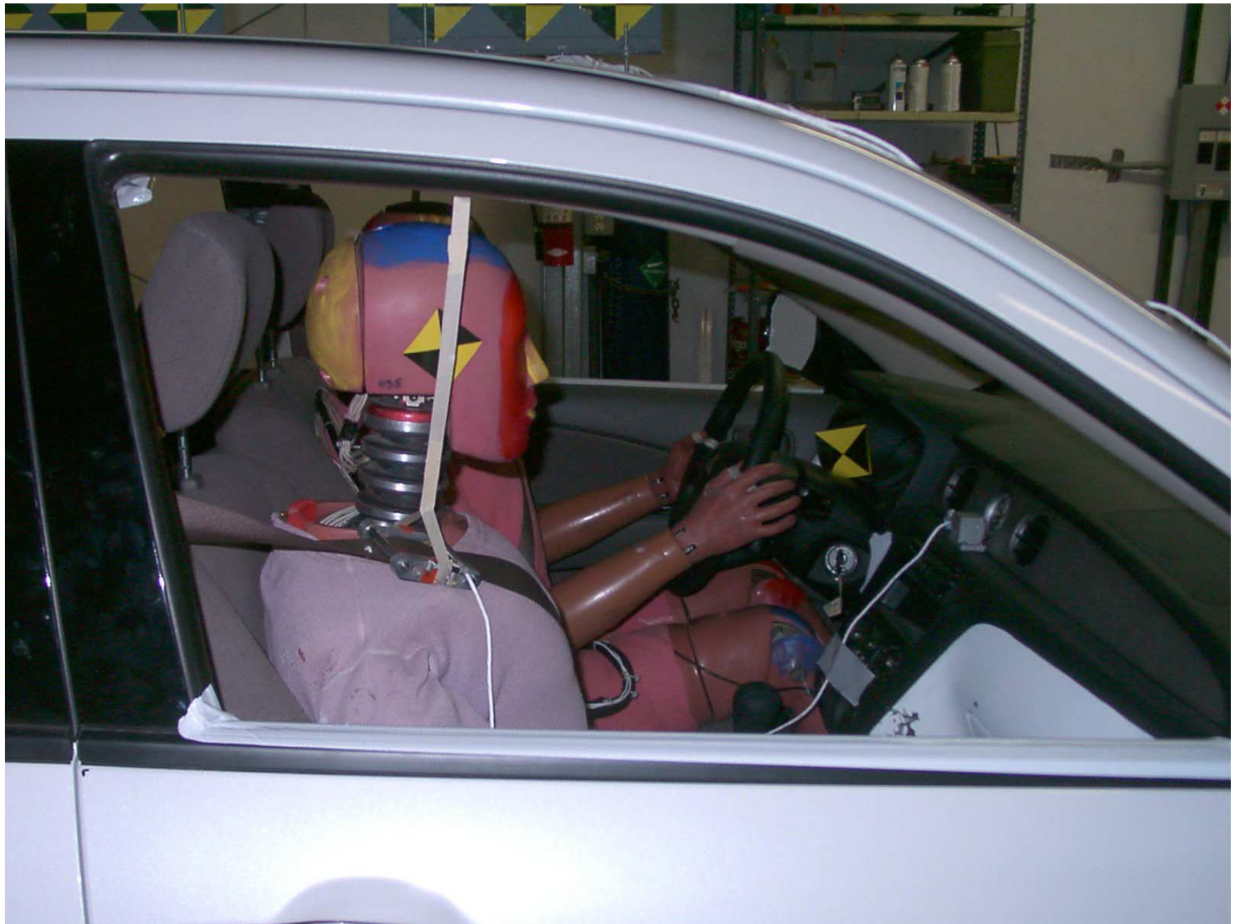
Figure A-46: Pre-Test Passenger Dummy Front Through Window
