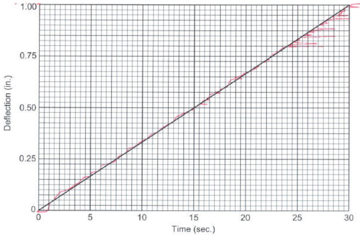
Compression - Deflection Resistance Test Child Seat Foam
