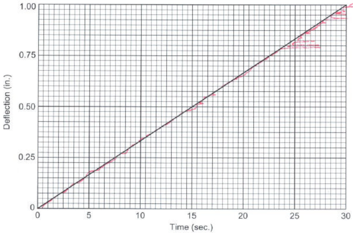
Compression - Deflection Resistance Test Child Seat Foam
