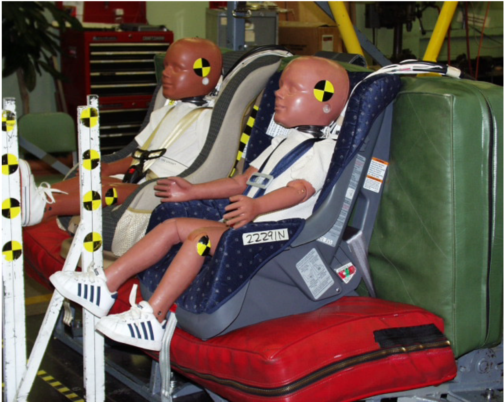
Run #22291 Photo 6 - Post-Test Left 3/4 View
