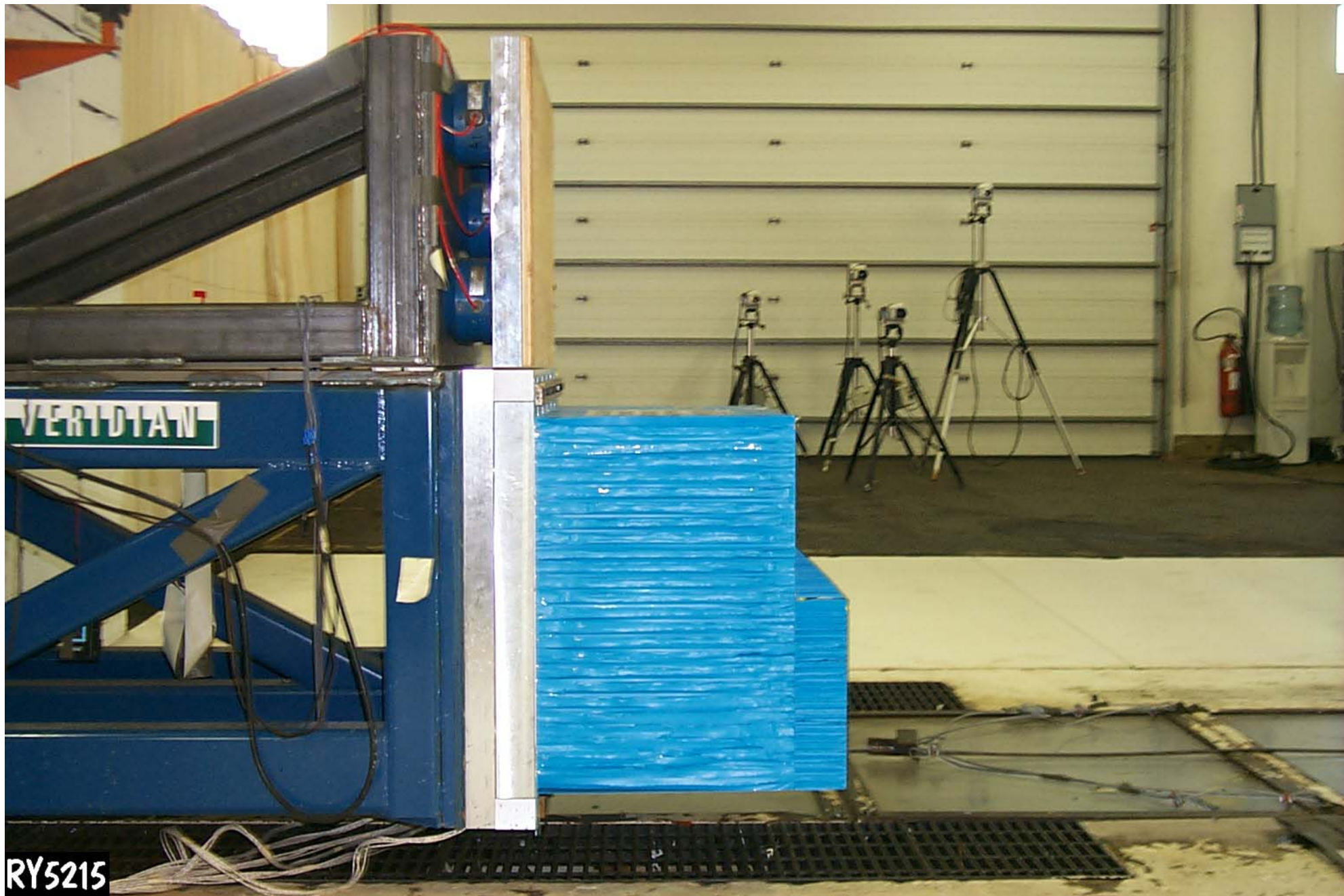
Figure A-39: PRE-TEST BARRIER LEFT SIDE VIEW
