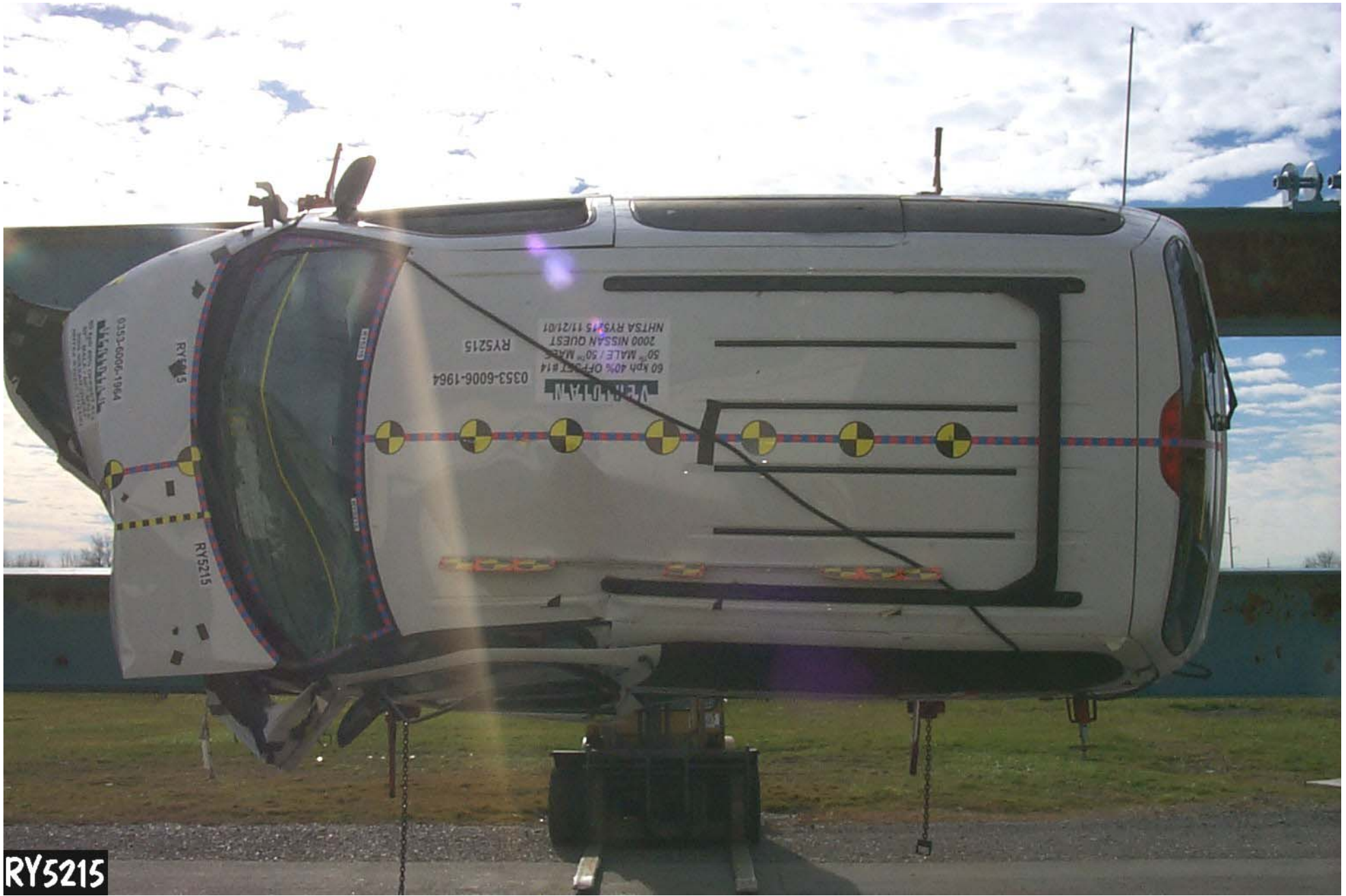
Figure A-46: ROLLOVER VIEW
