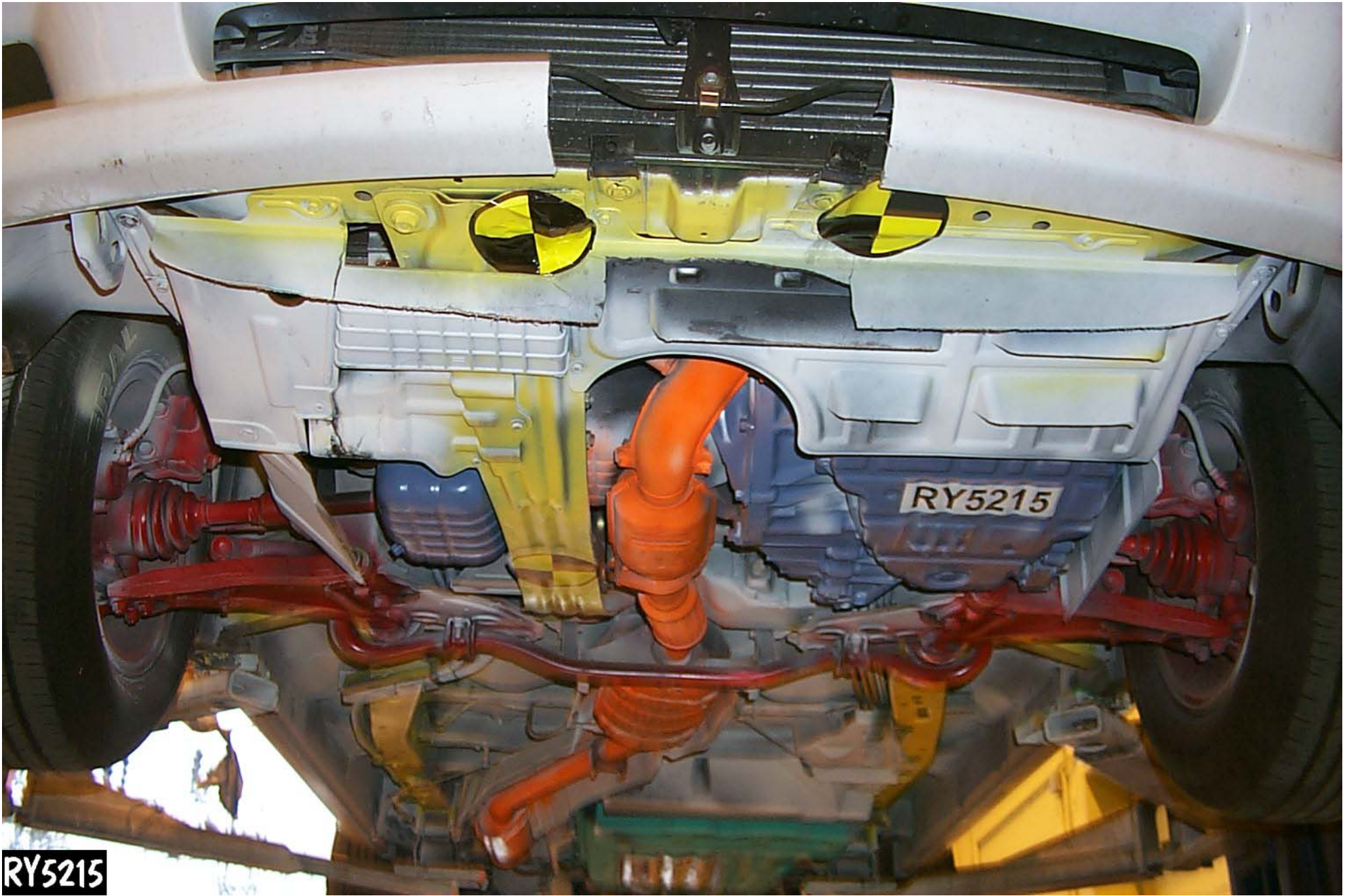
Figure A-15: PRE-TEST FRONT UNDERBODY VIEW
