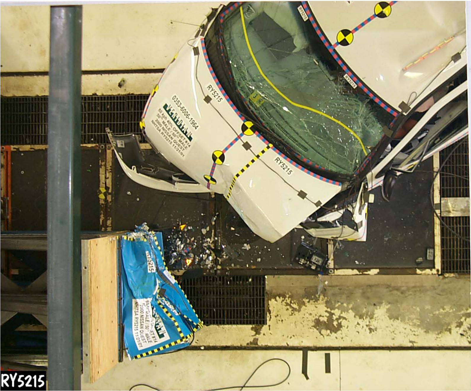
Figure A-45: POST-TEST OVERHEAD VIEW
