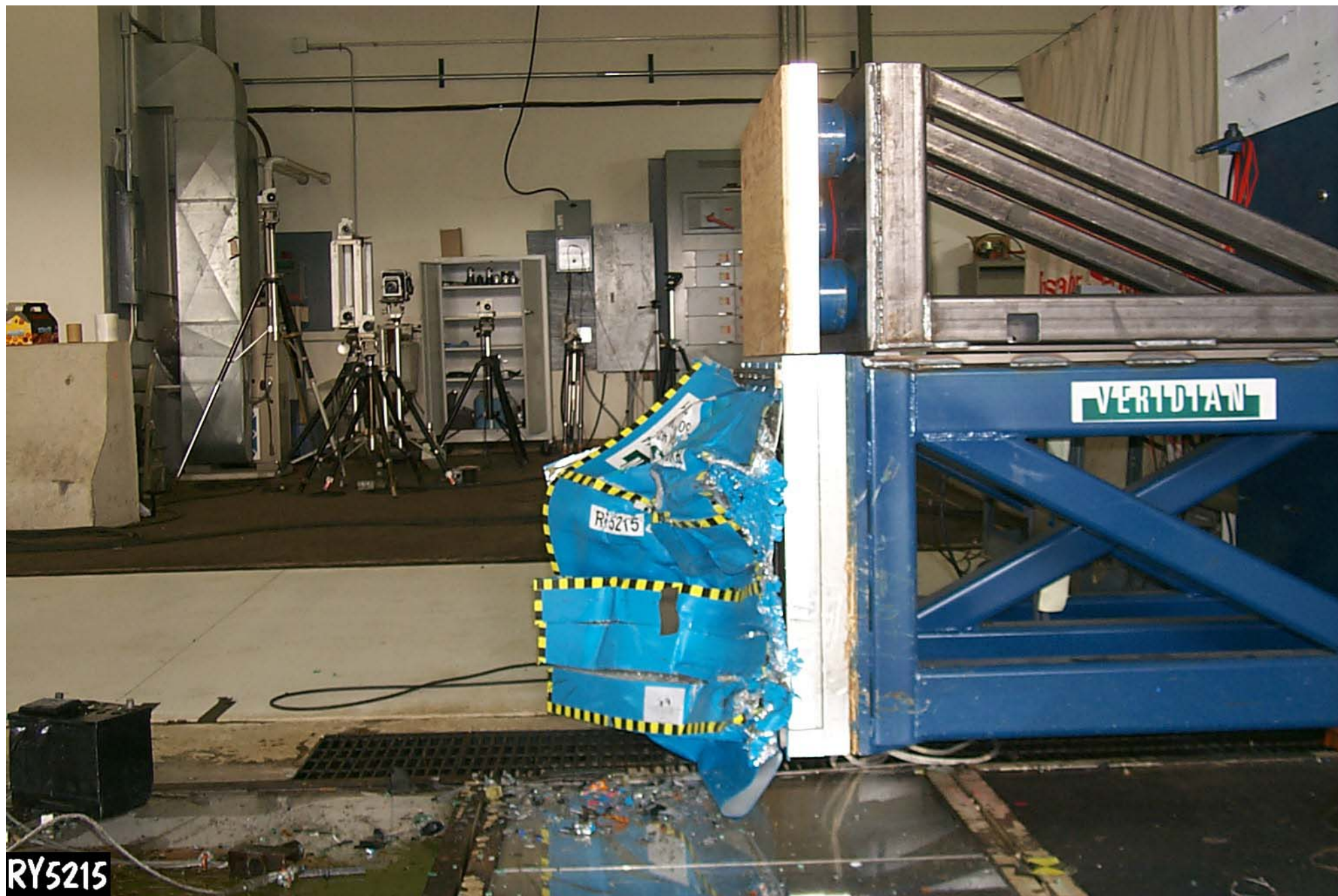
Figure A-42: POST-TEST BARRIER RIGHT SIDE VIEW
