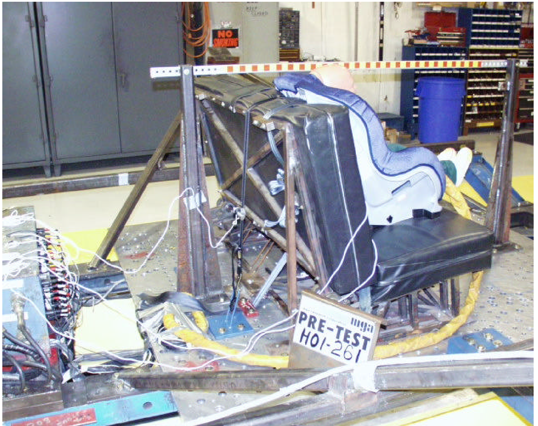
Photo 9 - Pre-Test Fixture
