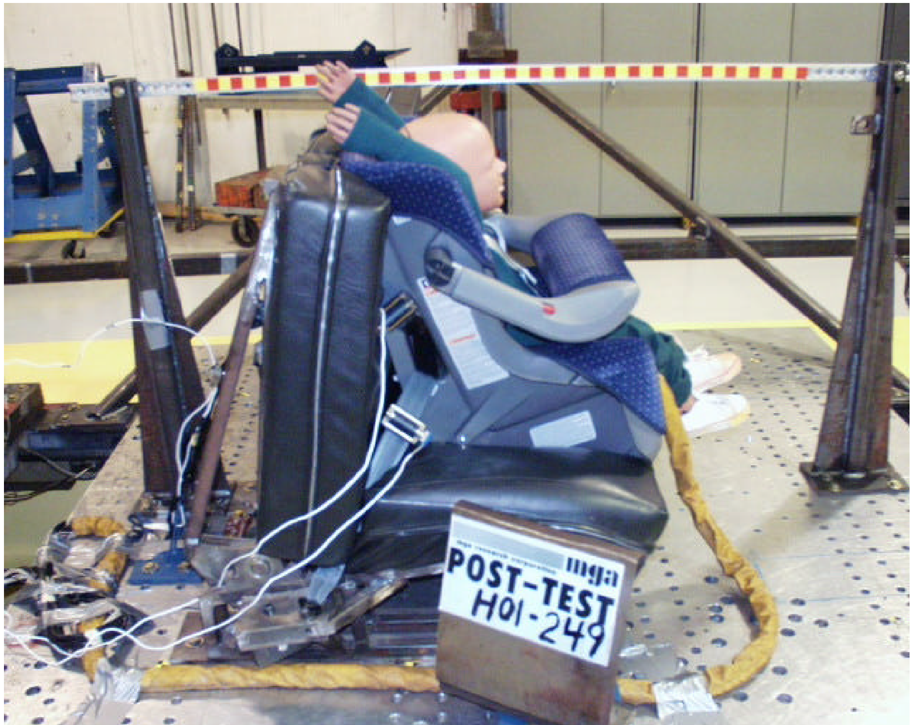
Photo 8 - Post-Test Right Side View
