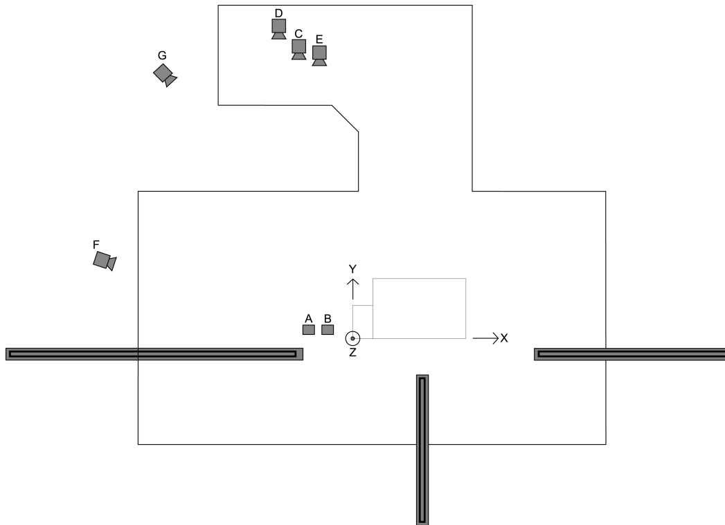
Figure 5 High-Speed Camera Positions
