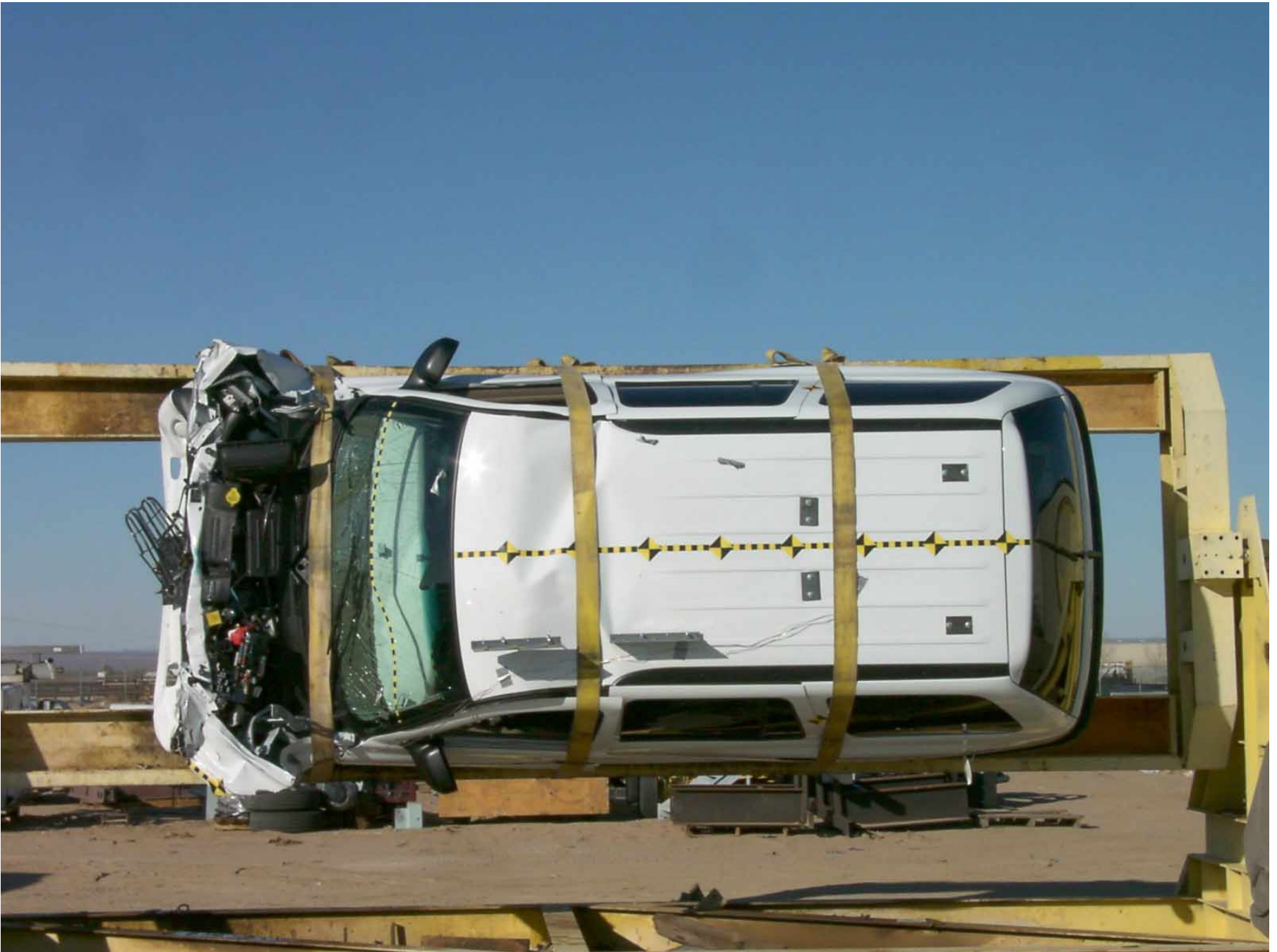
Figure A-57: Vehicle on Rollover Device
