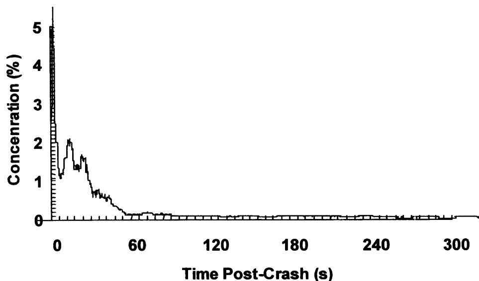
Figure 22 Concentration of Hydrocarbon Gas Measured near Left Exhaust Manifold (Location #3) Test C11591
