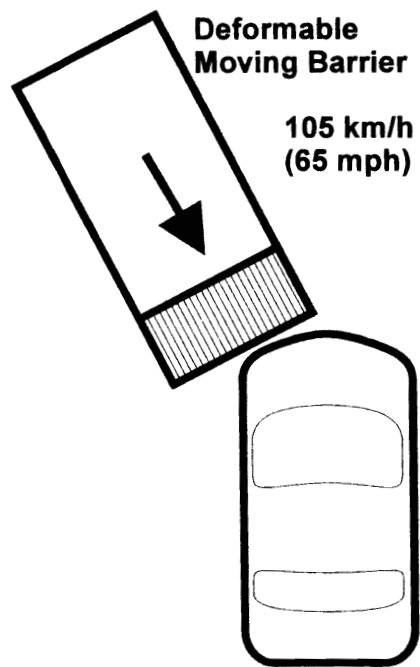
Figure 26 Crash Test Configuration for Test C11647
