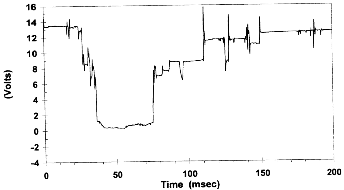
Figure 39 Ignition Voltage Test C11647
