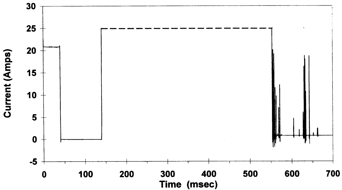
Figure 9 Rear Defroster Current, Test C11408
