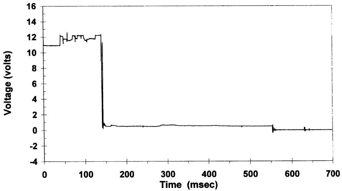
Figure 10 Rear Defroster Voltage, Test C11408
