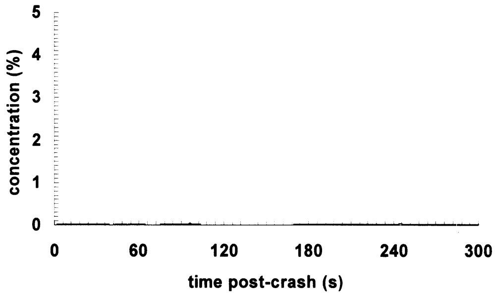
Figure H5 Concentration Of Hydrocarbon Vapor Measured Near The Catalytic Converter (Location #5) Test C11647
