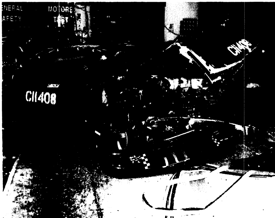
Figure 4 Post-Test Photograph of Test C11408, Left-Rear View
