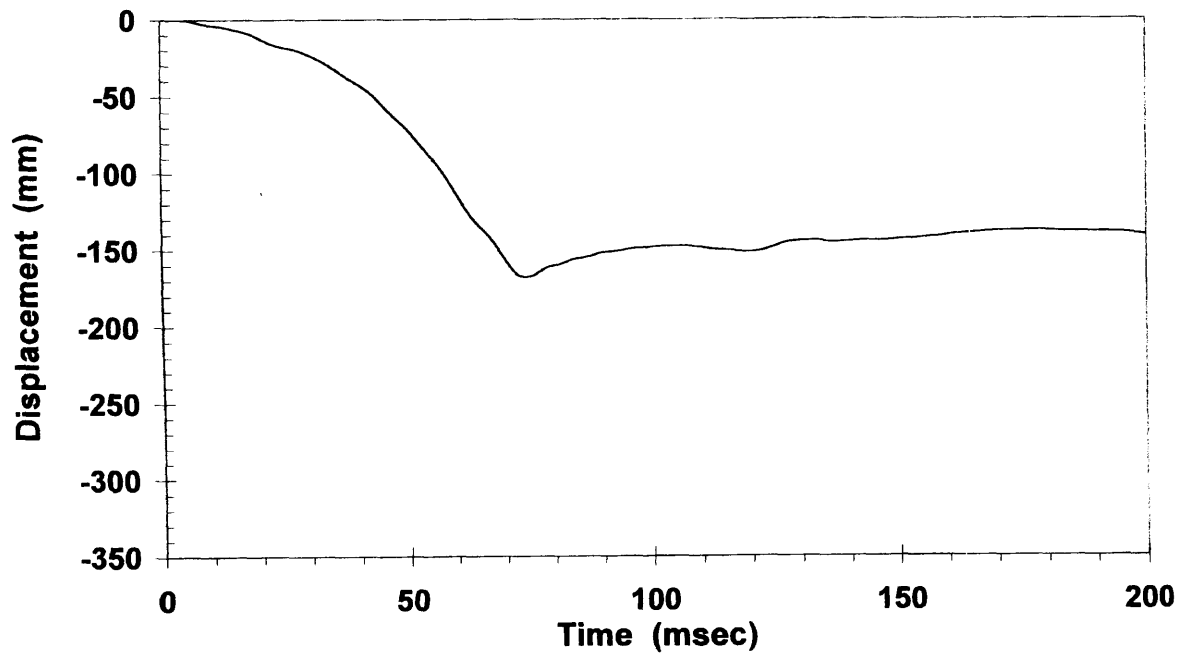
Figure 36 Left Toe Pan Displacement, Relative to Floorpan Test C11647, filtered at SAE class 60 [8]
