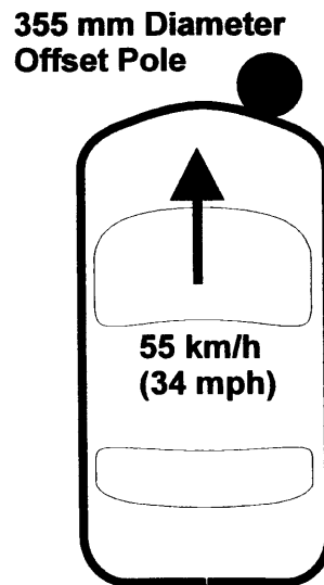
Figure 12 Crash Test Configuration for Test C11591
