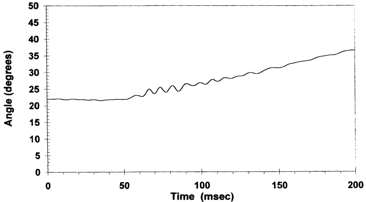
Figure 32 Vehicle's Yaw Angle, \theta(t) Test C11647
