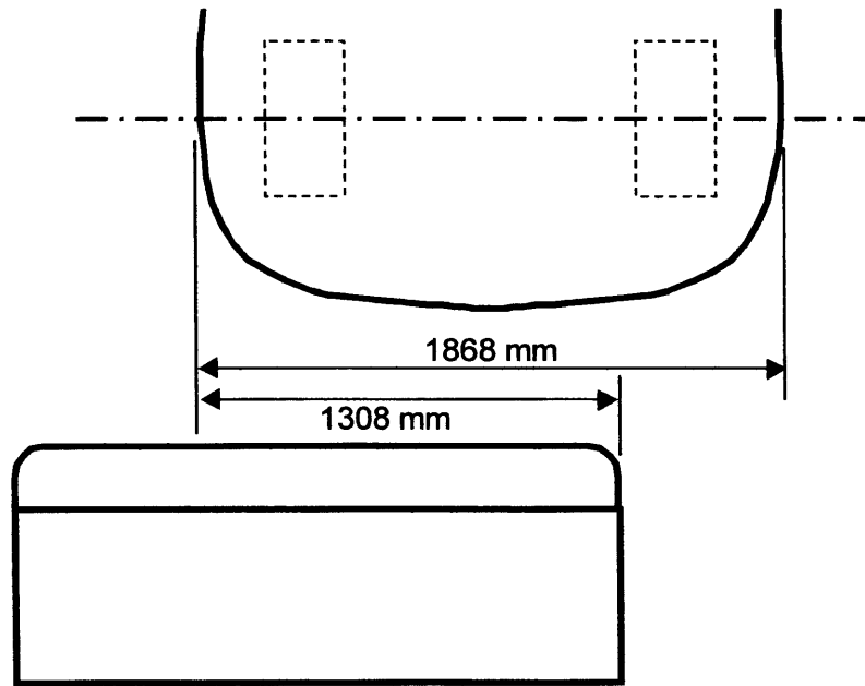
Figure 3 Schematic of Intended Vehicle Overlap Test C11408
