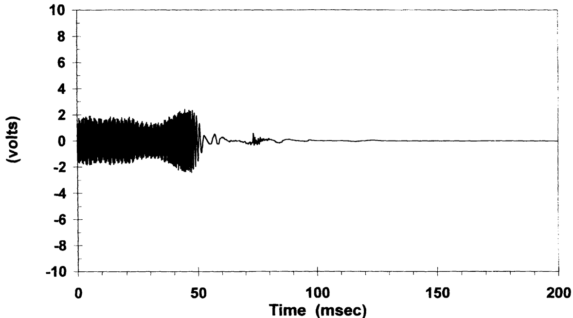
Figure 37 Engine Motion Measured using Auxiliary Magnetic Pickup Transducer, Test C11647
