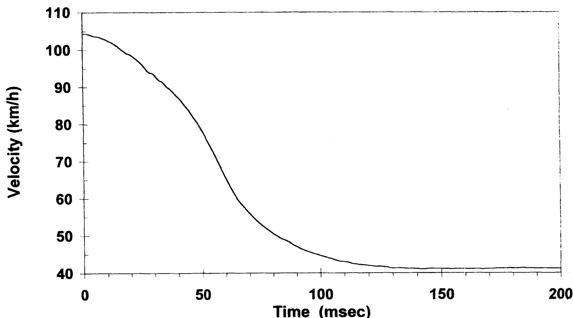
Figure 40 Moving Deformable Barrier Longitudinal Velocity at CG Test C11647
