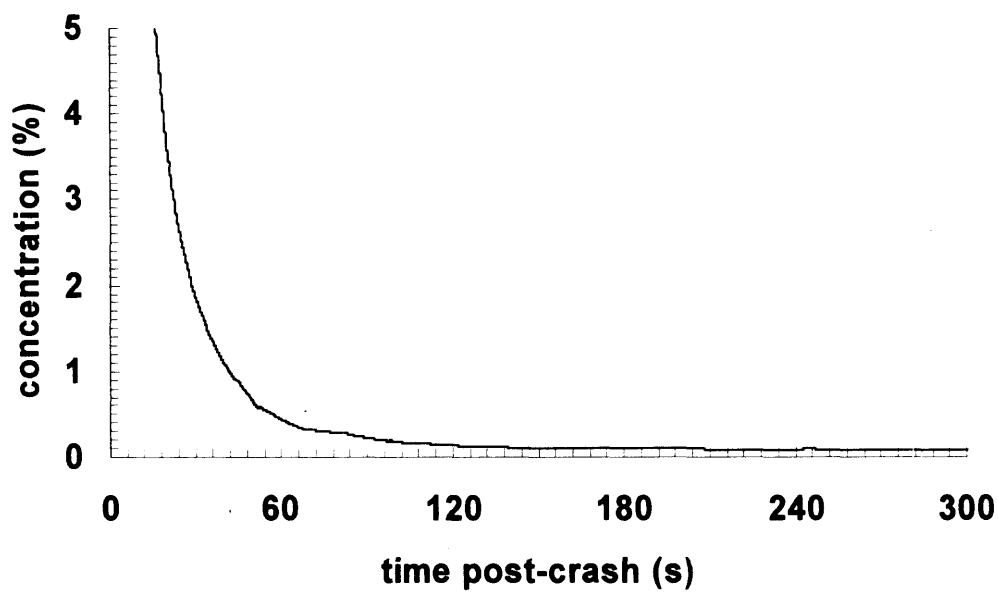
Figure H2 Concentration of Hydrocarbon Vapor Measured above the Left Exhaust Manifold (Location #2) Test C11647
