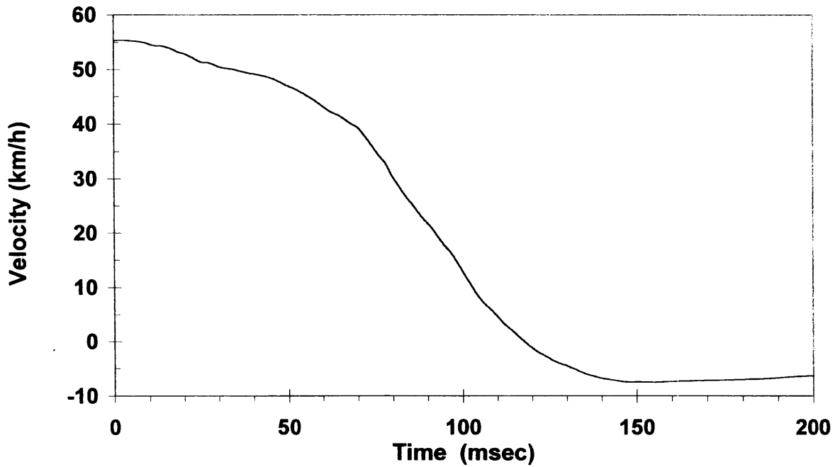
Figure 18 Averaged (Left & Right) Rear Rocker Panel Longitudinal Velocity Test C11591
