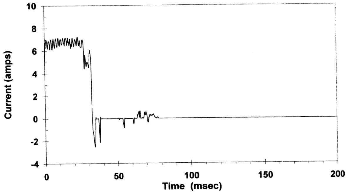
Figure 38 Fuel Pump Current Test C11647
