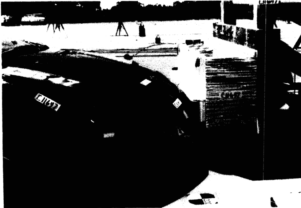
Figure 26 Crash Test Configuration for Test C11647
