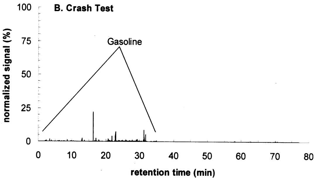
Figure EE5 GC/FID analysis of hydrocarbon vapor sample near catalytic converter (location #5) during Crash Test C11591. Panel A shows the chromatogram of background sample and panel B shows the chromatogram of the post-crash sample.
