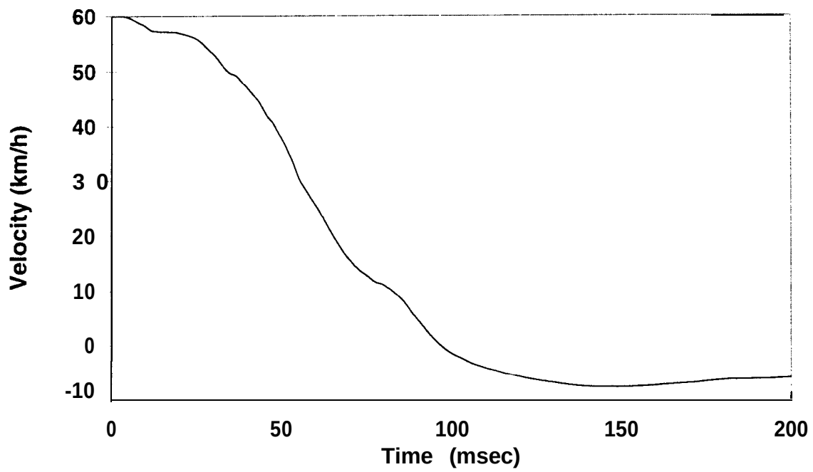
Figure 35 Averaged (Left & Right) Rear Rocker Panel Longitudinal Velocity Test CI 1226
