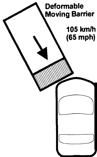
Figure 11. Crash Test Configuration for Test CI 1167
