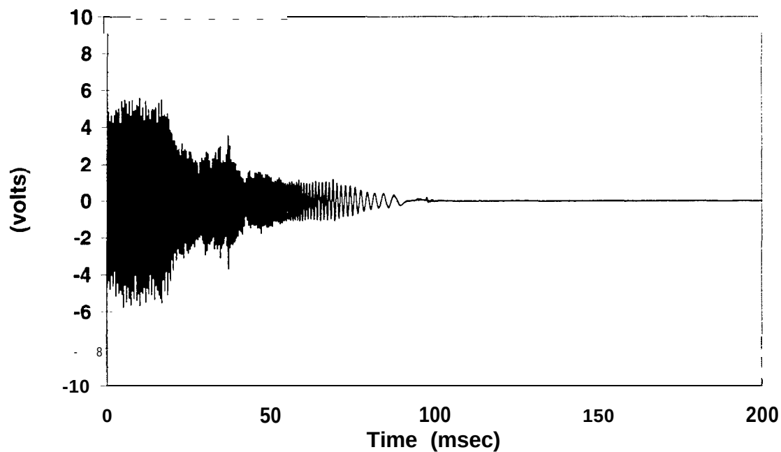
Figure 46 Engine Motion, Measured at Flywheel Test CI 1279
