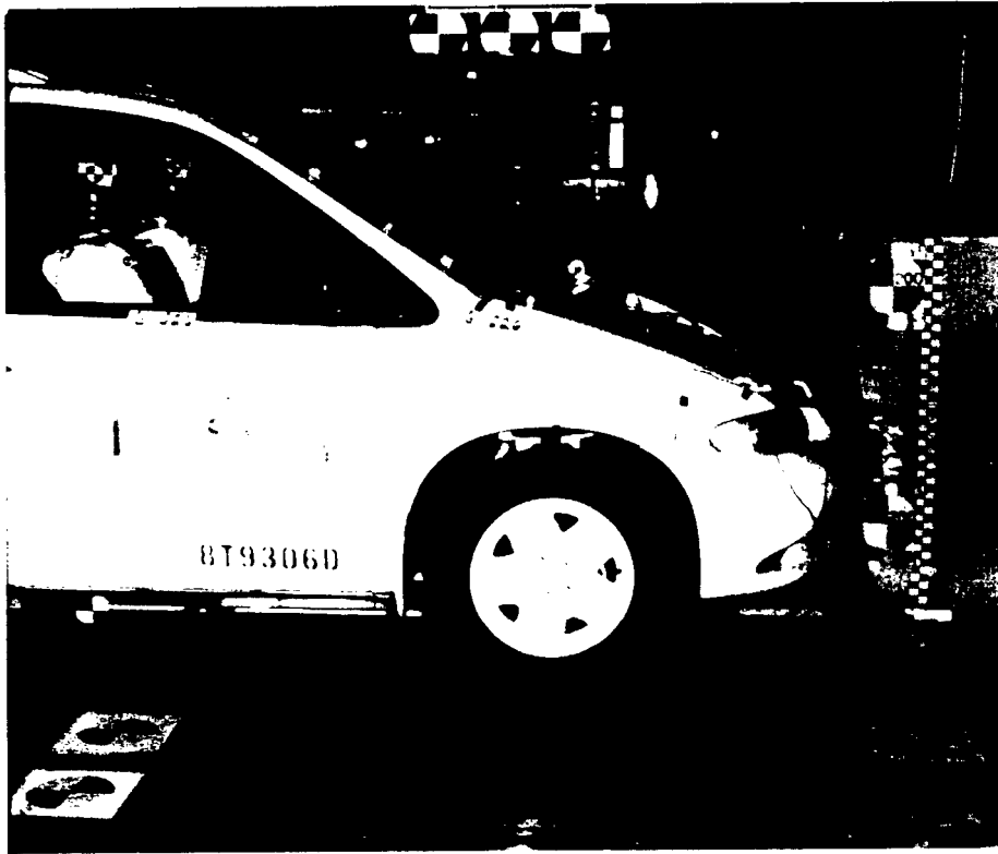
Figure 31. Pre-Test Photograph of Test CI 1226
