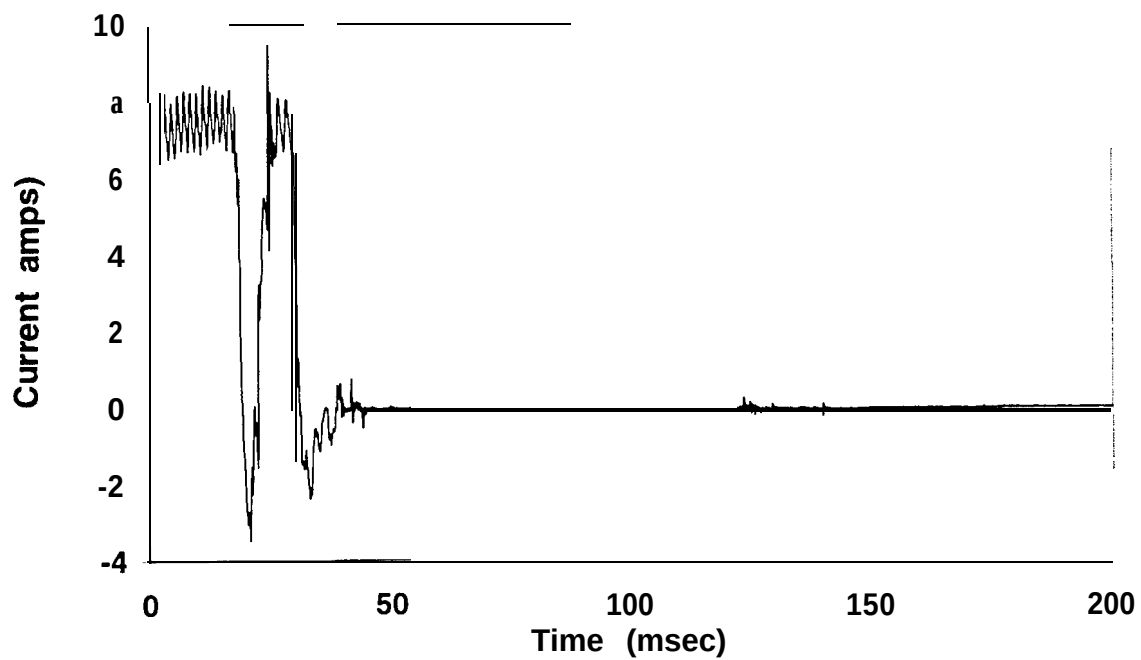
Figure 37 Fuel Pump Current Test CI 1226
