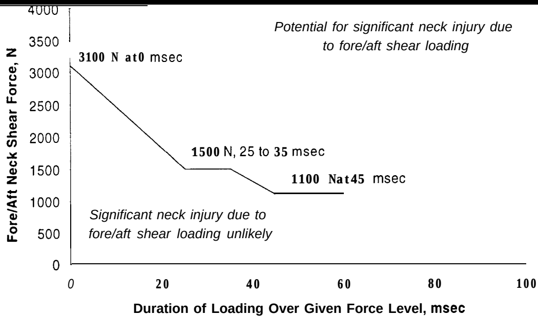
Figure A1 Injury Assessment Curves for Fore-and-Aft Shear Forces Measured with Hybrid III Mid-sized Adult Male ATD [5]
