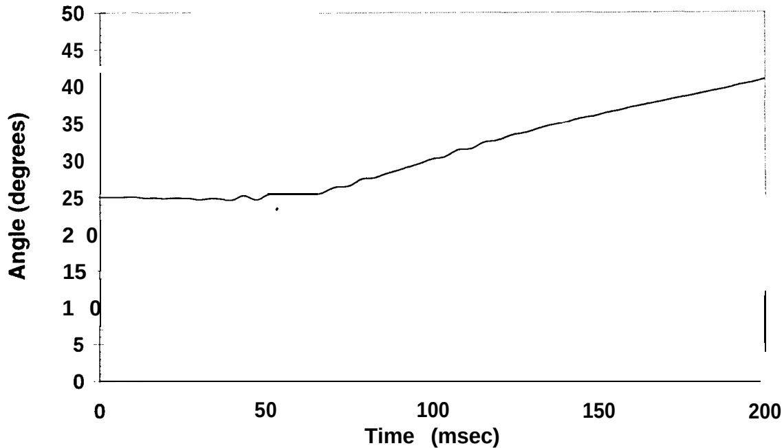
Figure 16. Vehicle's Yaw Angle, \theta(T) Test CI 1167
