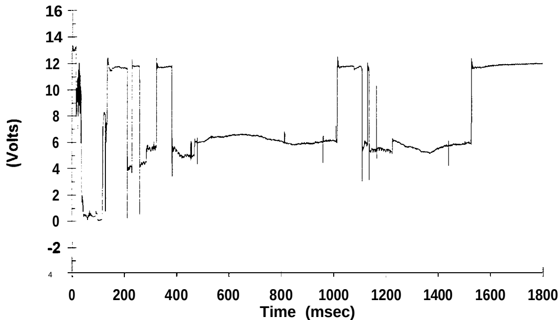
Figure 21 Ignition Voltage Test CI 1167
