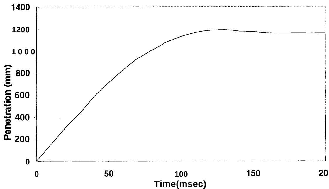
Figure 54. Pole Penetration Test CI 1279, Numerically Measured from High Speed Film
