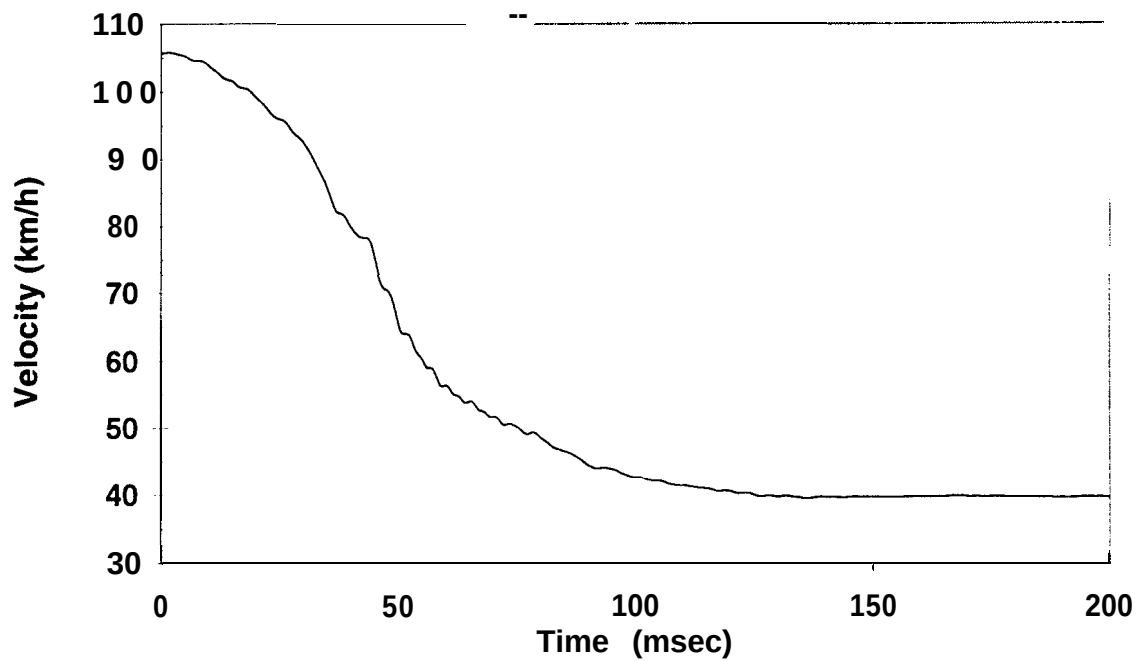
Figure 23 Moving Deformable Barrier Longitudinal Velocity at CG Test CI1167
