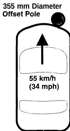
Figure 39. Crash Test Configuration for Test CI 1279
