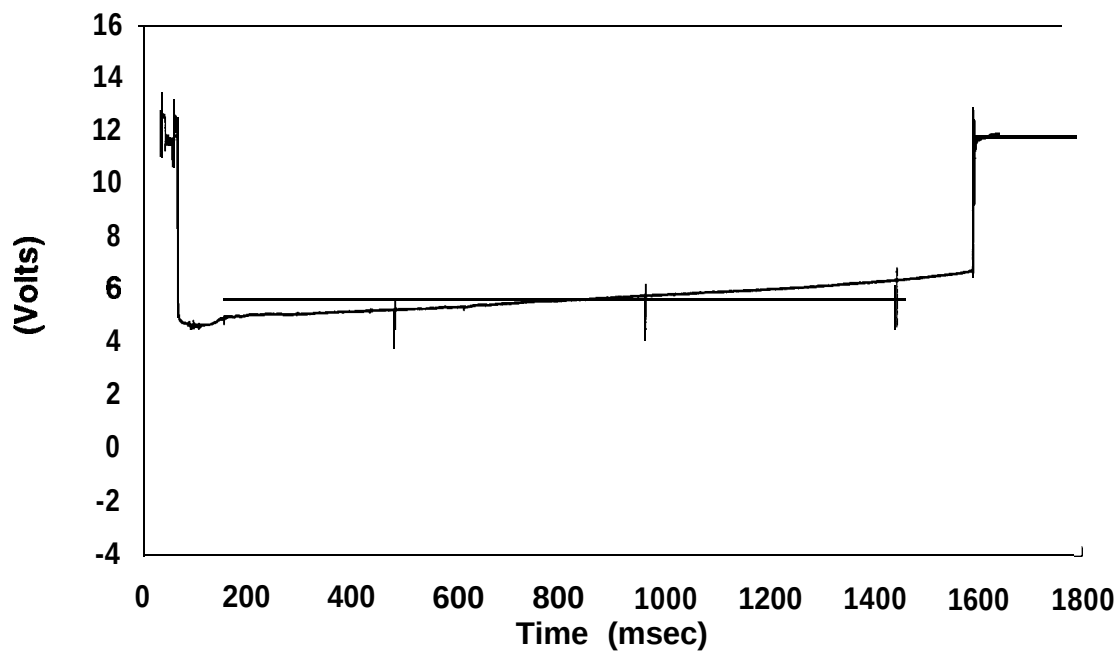
Figure 48 Ignition Voltage Test CI 1279
