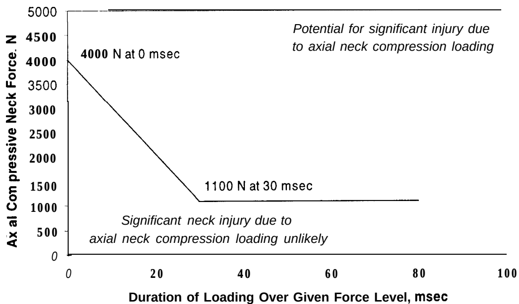
Figure A2 Injury Assessment Curves for Axial Neck Compression Measured with Hybrid III Mid-sized Adult Male ATD [5]
