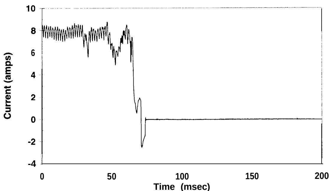
Figure 8 Fuel Pump Current Test CI 1108
