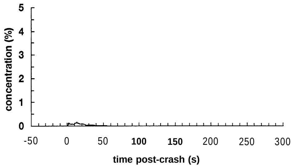
Figure 15 Concentration of Hydrocarbon Vapor Measured at Exhaust Manifold (Location #5) TestC11279
