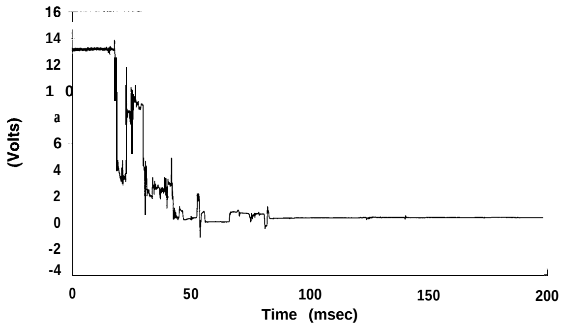
Figure 38 Ignition Voltage Test CI 1226
