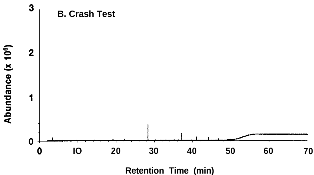
Figure EE4 GC/MS analysis of hydrocarbon vapor sampled from the right lower engine (location #4) during Crash Test C11167. Panel A shows the chromatogram of a background sample and panel B shows the chromatogram of the post-crash sample.
