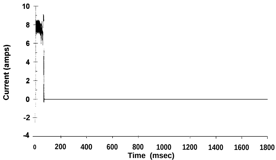
Figure 47 Fuel Pump Current Test CI 1279
