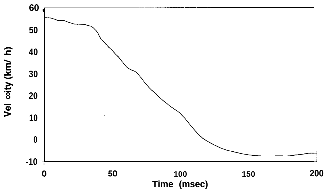
Figure 44 Averaged (Left & Right) Rear Rocker Panel Longitudinal Velocity Test CI 1279
