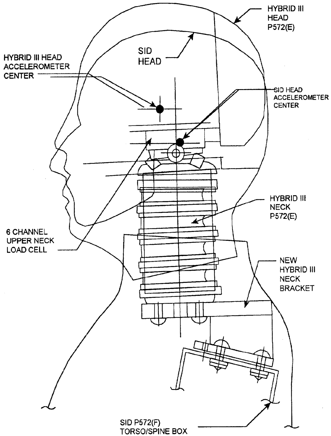
Figure 2. HYBRID III neck and head assembly on SID/HIII #28.
