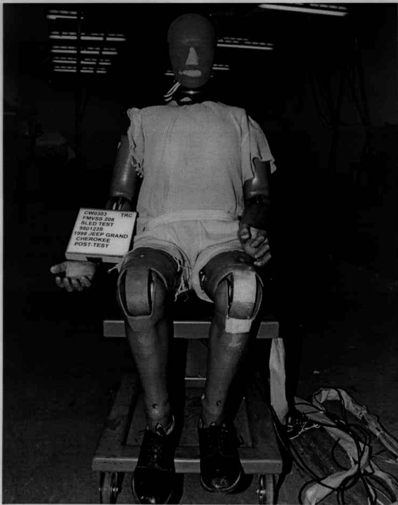
Figure A-31 Post-Test Passenger Dummy Removed From Vehicle Overall View A-32 980123
