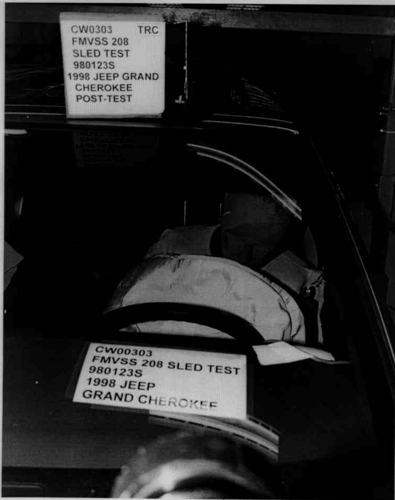
Figure A-16 Post-Test Driver Dummy Position Front View A-17
