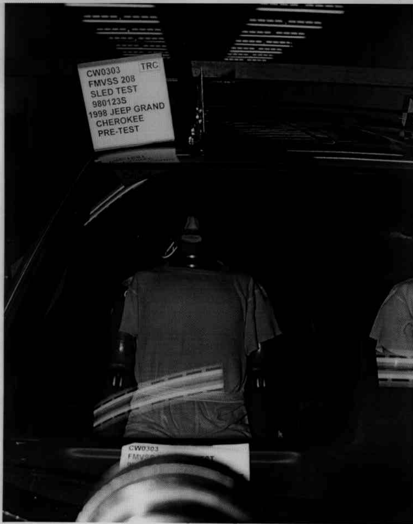
Figure A-28 Pre-Test Passenger Dummy Position Front View A-29
