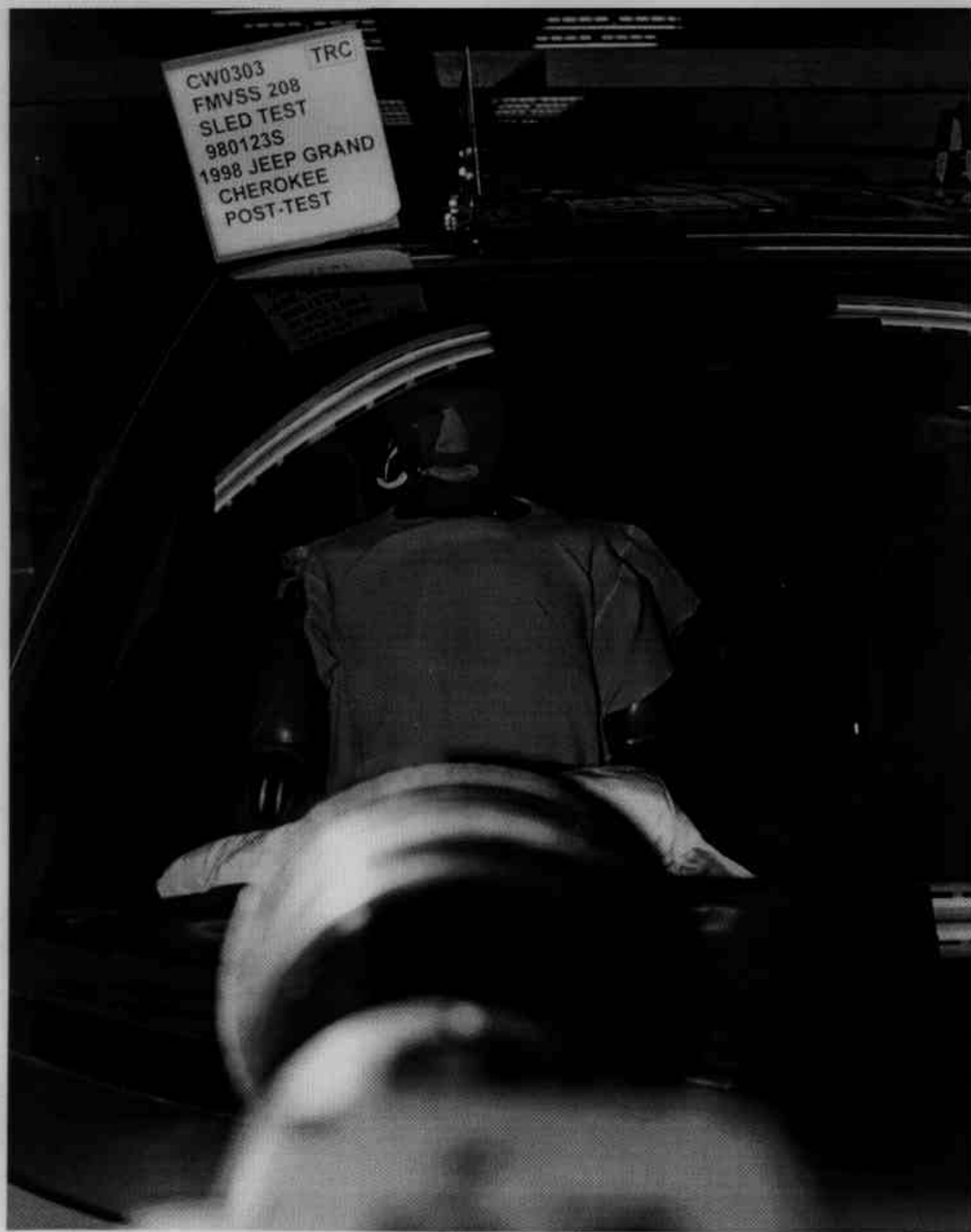
Figure A-29 Post-Test Passenger Dummy Position Front View A-30
