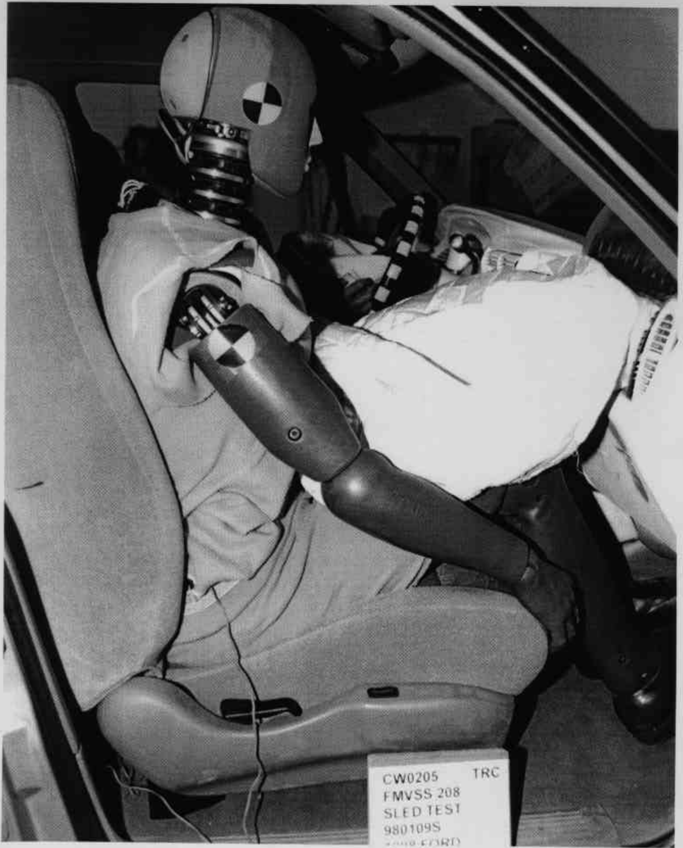
Figure A-19 Post-Test Passenger Dummy Position View With Door Open
