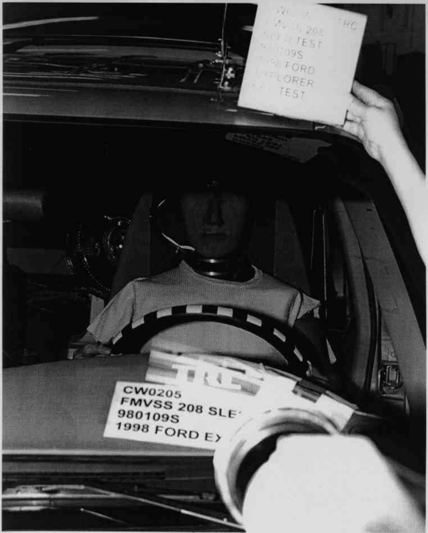
Figure A-13 Pre-Test Driver Dummy Position Front View A-14
