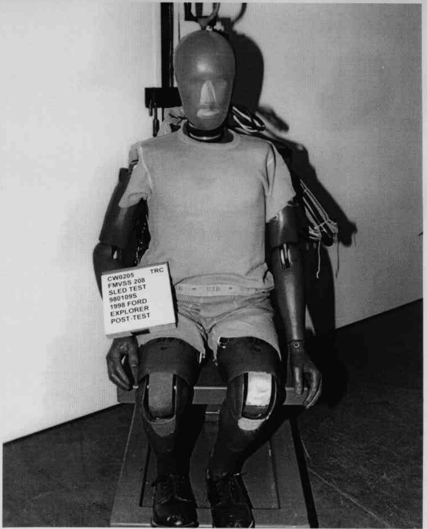
Figure A-29 Post-Test Passenger Dummy Overall View
