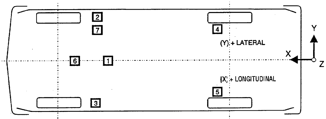
BOTTOM VIEW
