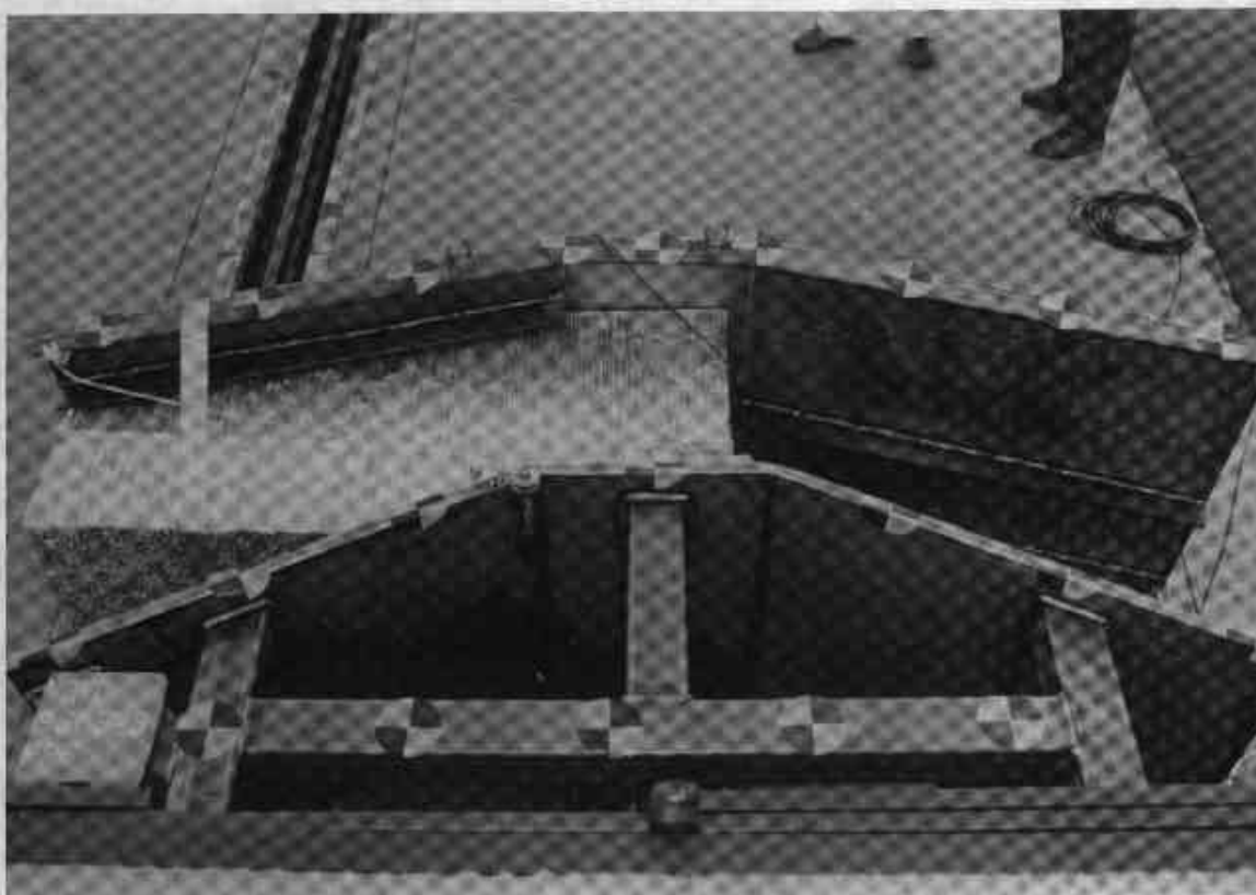
Figure A-24 Pre-Test Truck Bumper - View 3
