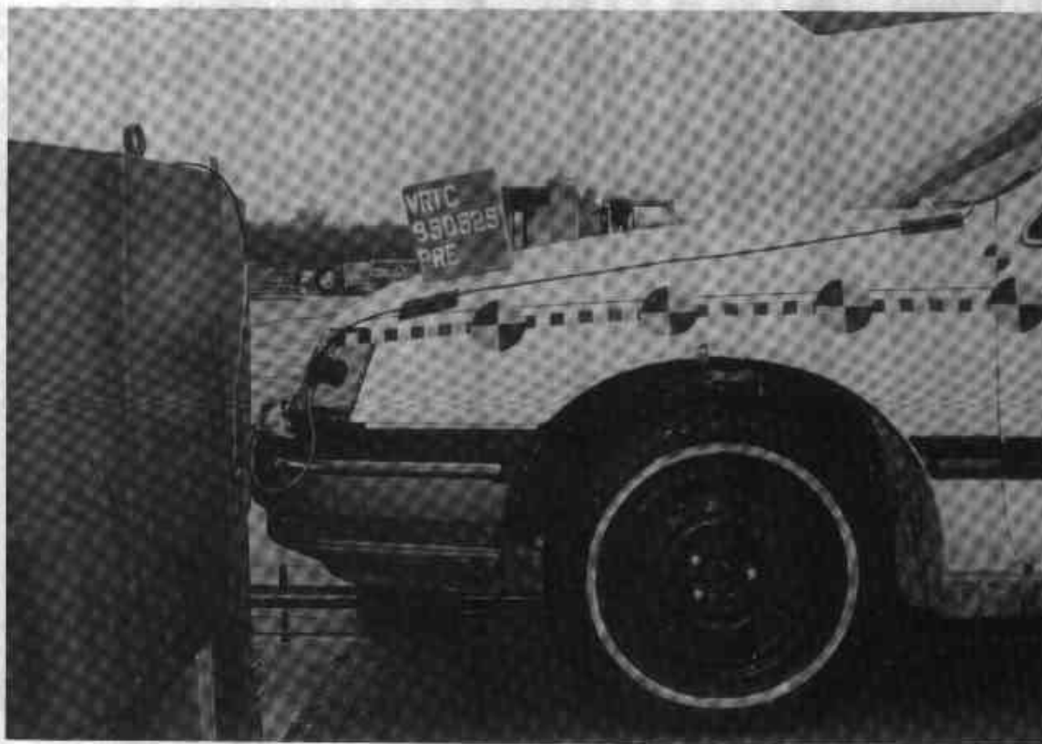
Figure A-18 Pre-Test Vehicle and Truck Bumper Engagement - View 1
