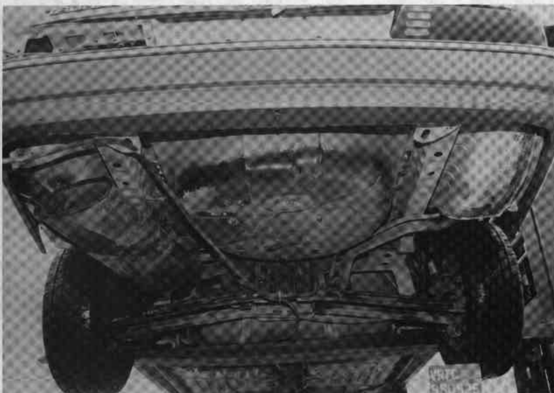
Figure A-17 Post-Test Rear Underbody View
