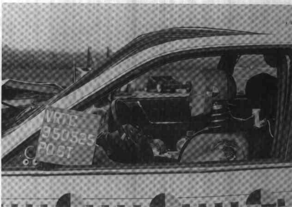
Figure A-26 Post-Test Driver Dummy - View 1
