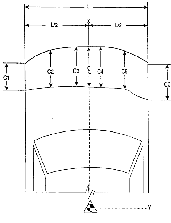
Figure 2 Vehicle Crush
