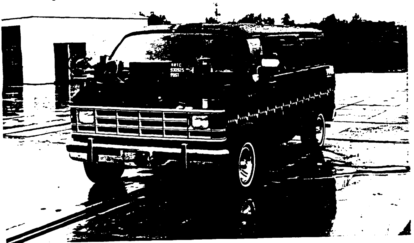
Figure A-14. POST-TEST LEFT FRONT THREE-QUARTER VIEW
