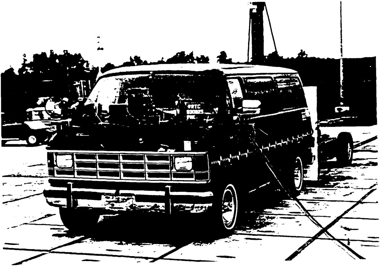
Figure A-13. PRE-TEST LEFT FRONT THREE-QUARTER VIEW
