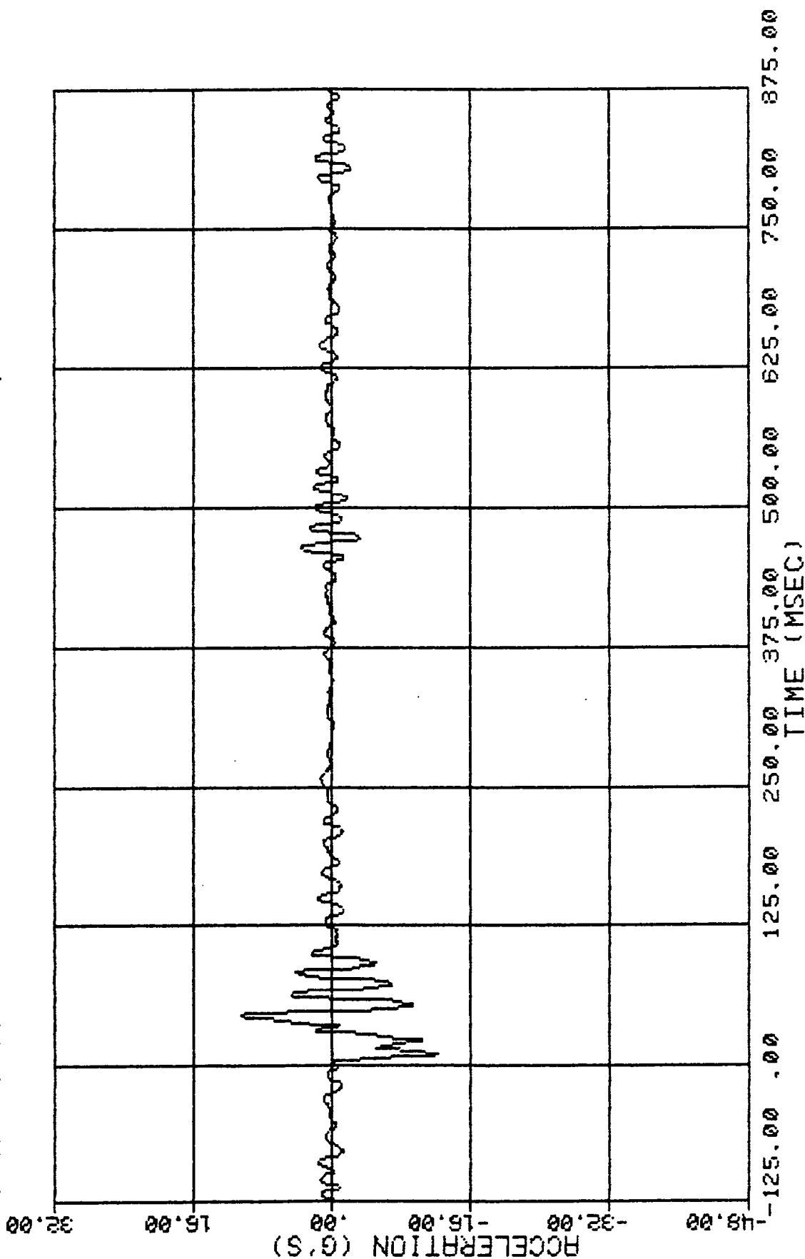
Figure A2. Vehicle Acceleration, Y-Axis, 100 Hz
