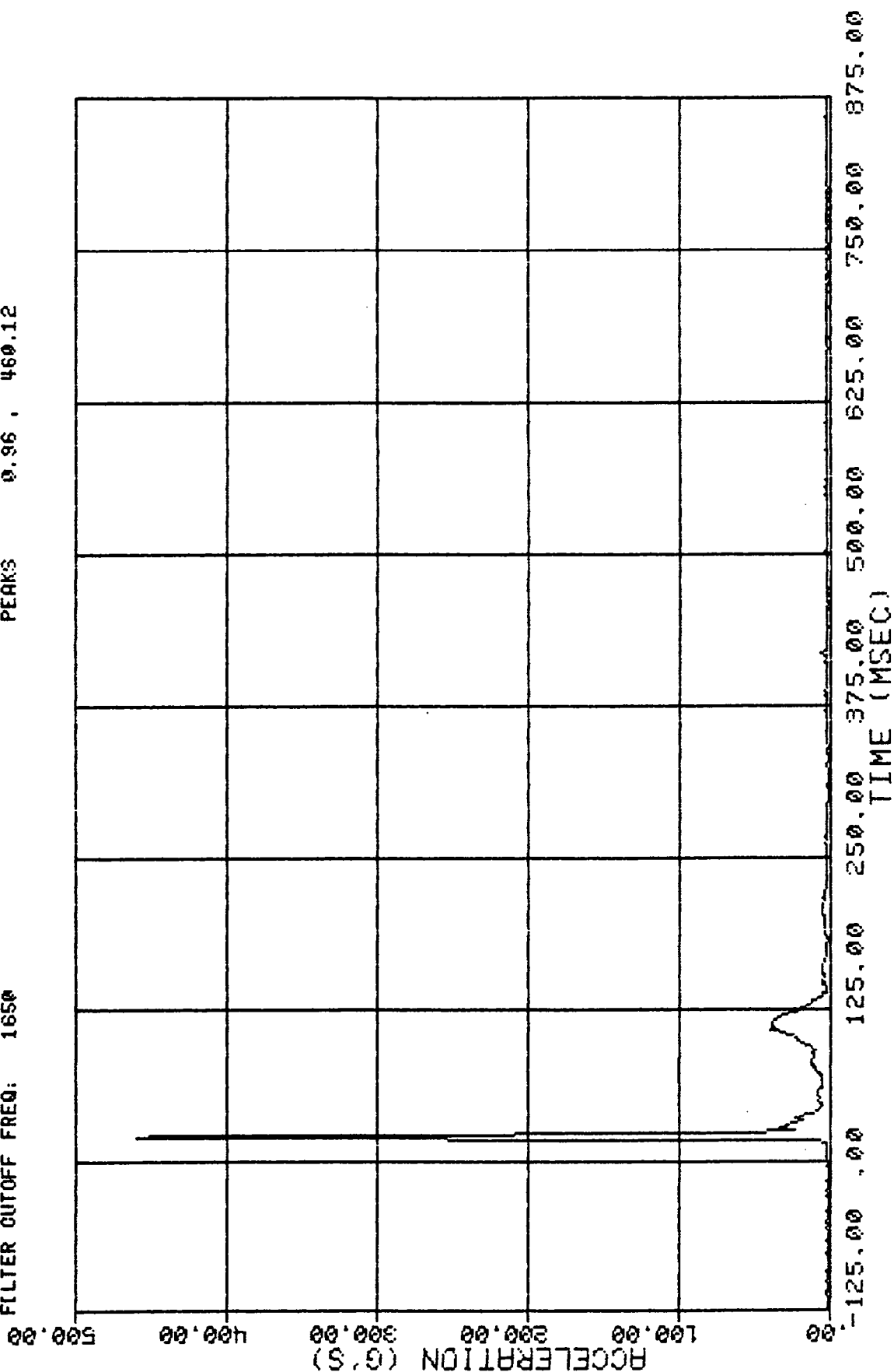
Figure A17. Driver's Head Acceleration, Resultant, 1650 Hz
