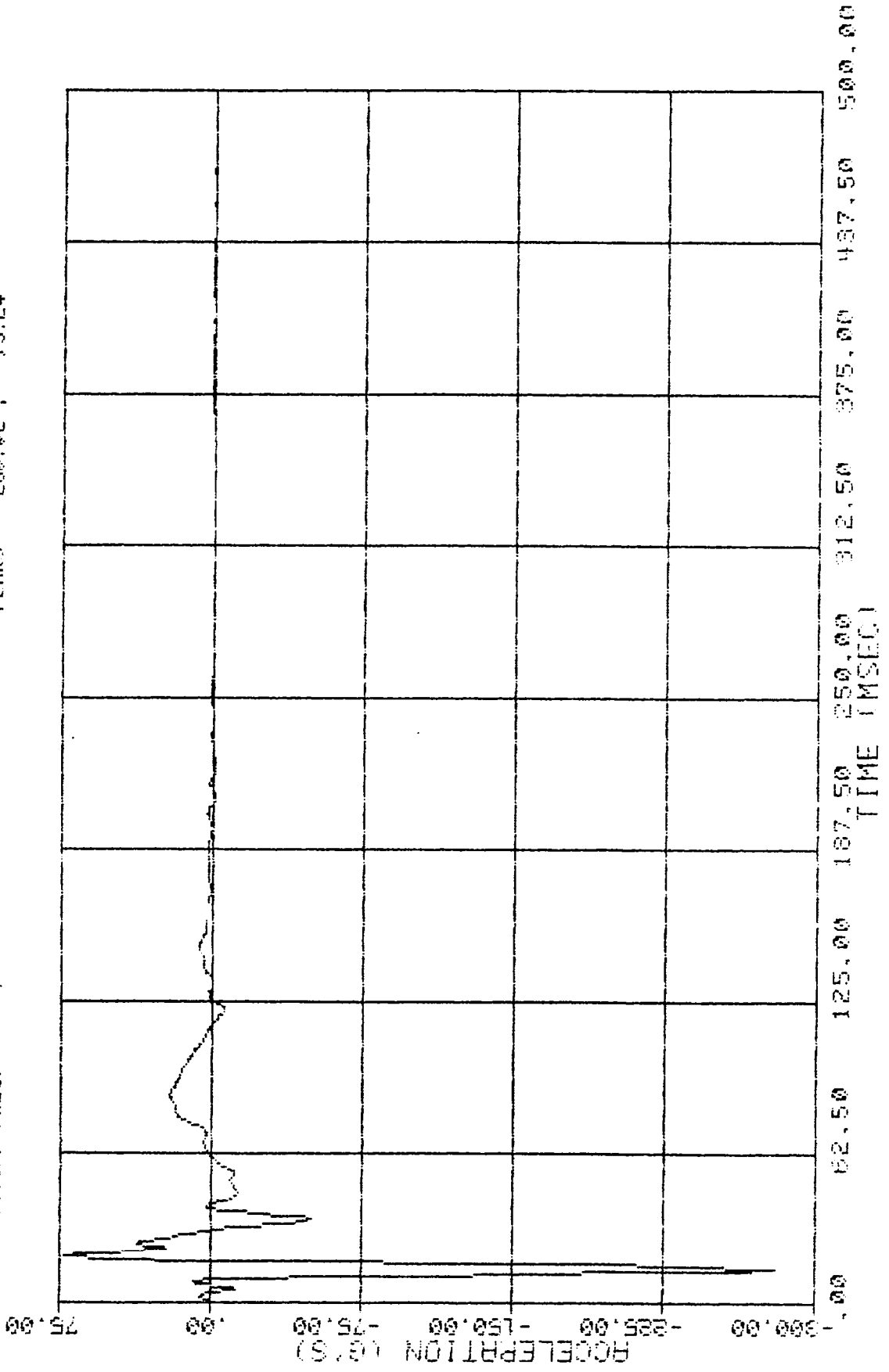
Figure A37. Driver's Left Upper Rib (LURY01) Acceleration, NHTSAFIR Filter
