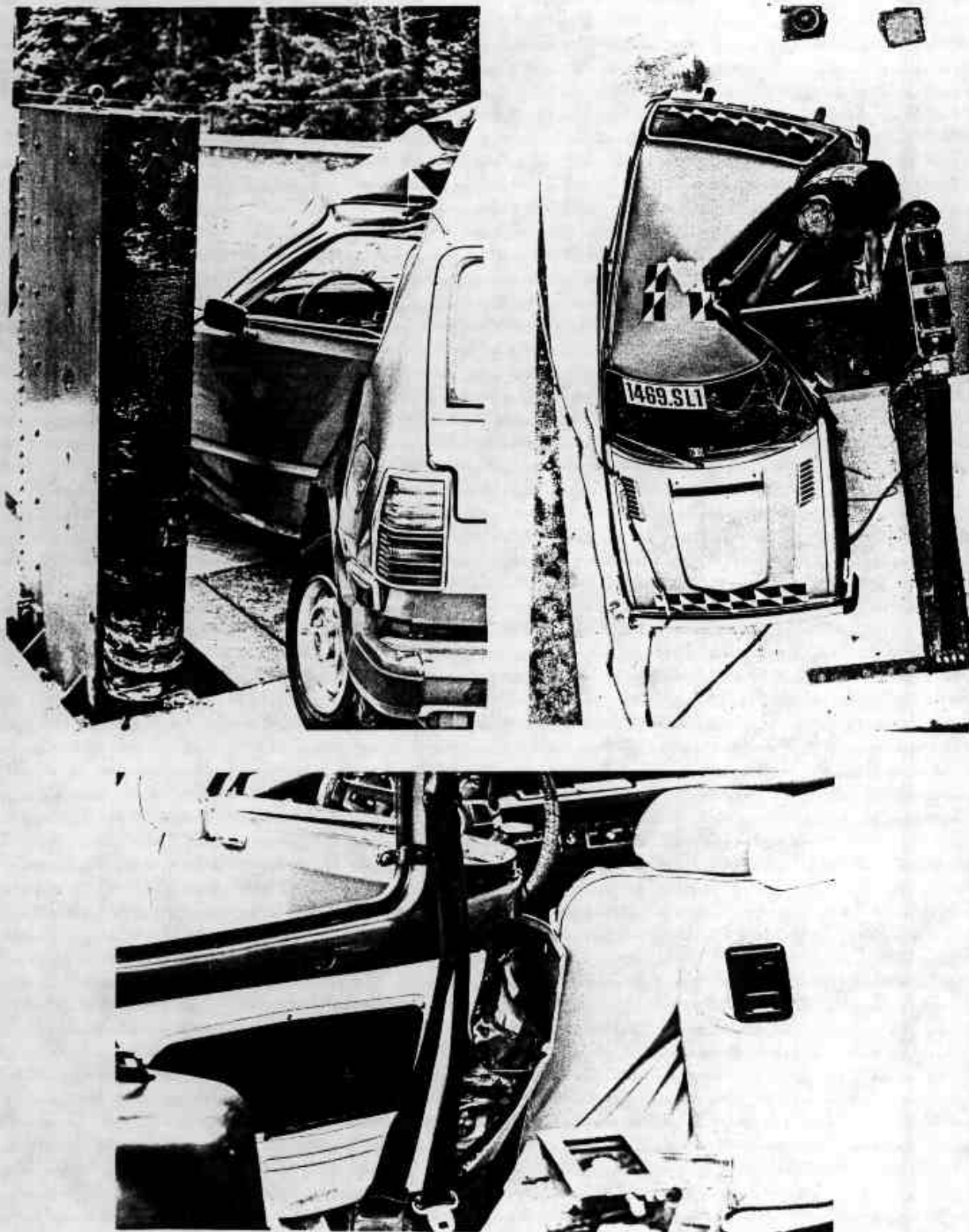
Figure 8. Post-Test Photos for Test 1469-SI#1
