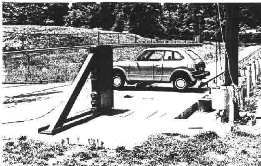
Figure 6. Pre-Test Photos for Test 1469-SI#1
