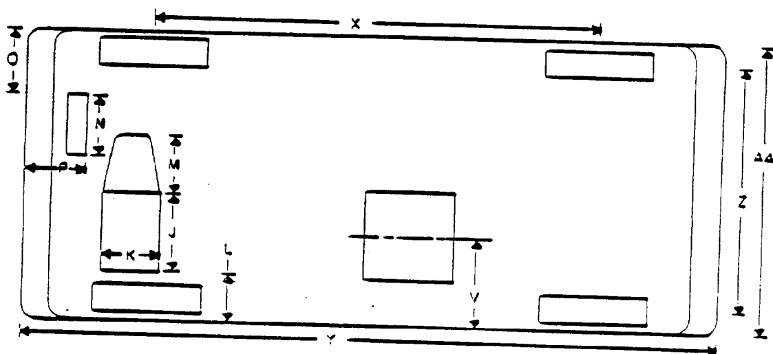
Figure 1. Key Dimensions for 1974-1979 Honda Civic
