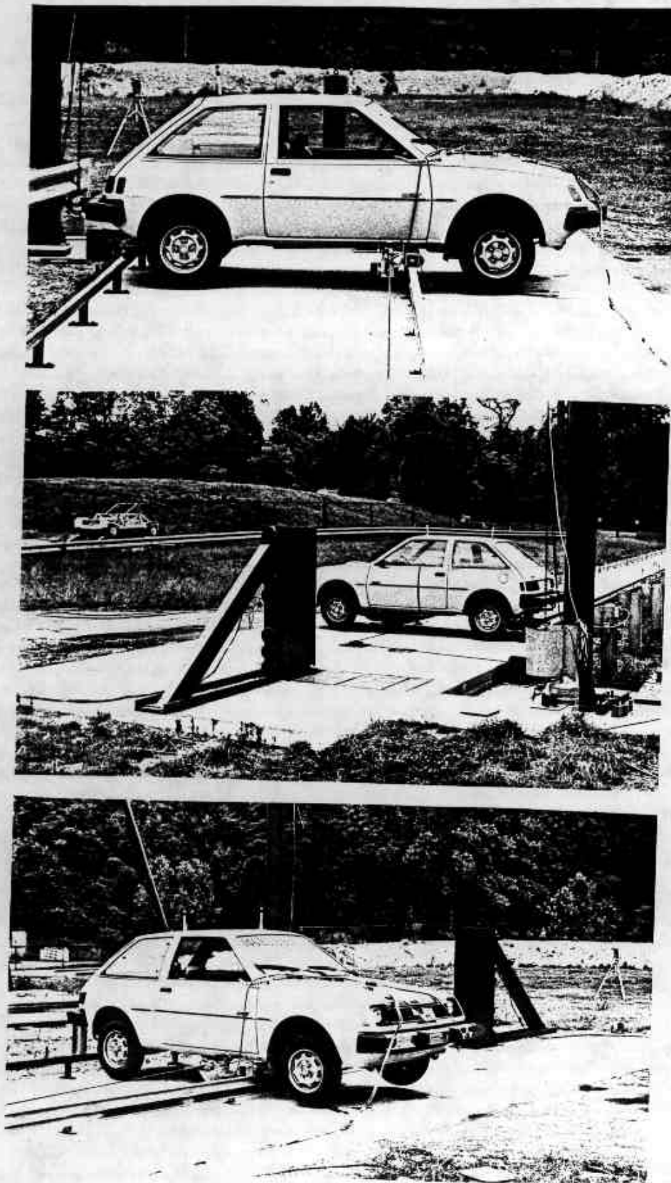
Figure 12. Pre-Test Photos for Test 1469-SI#3
