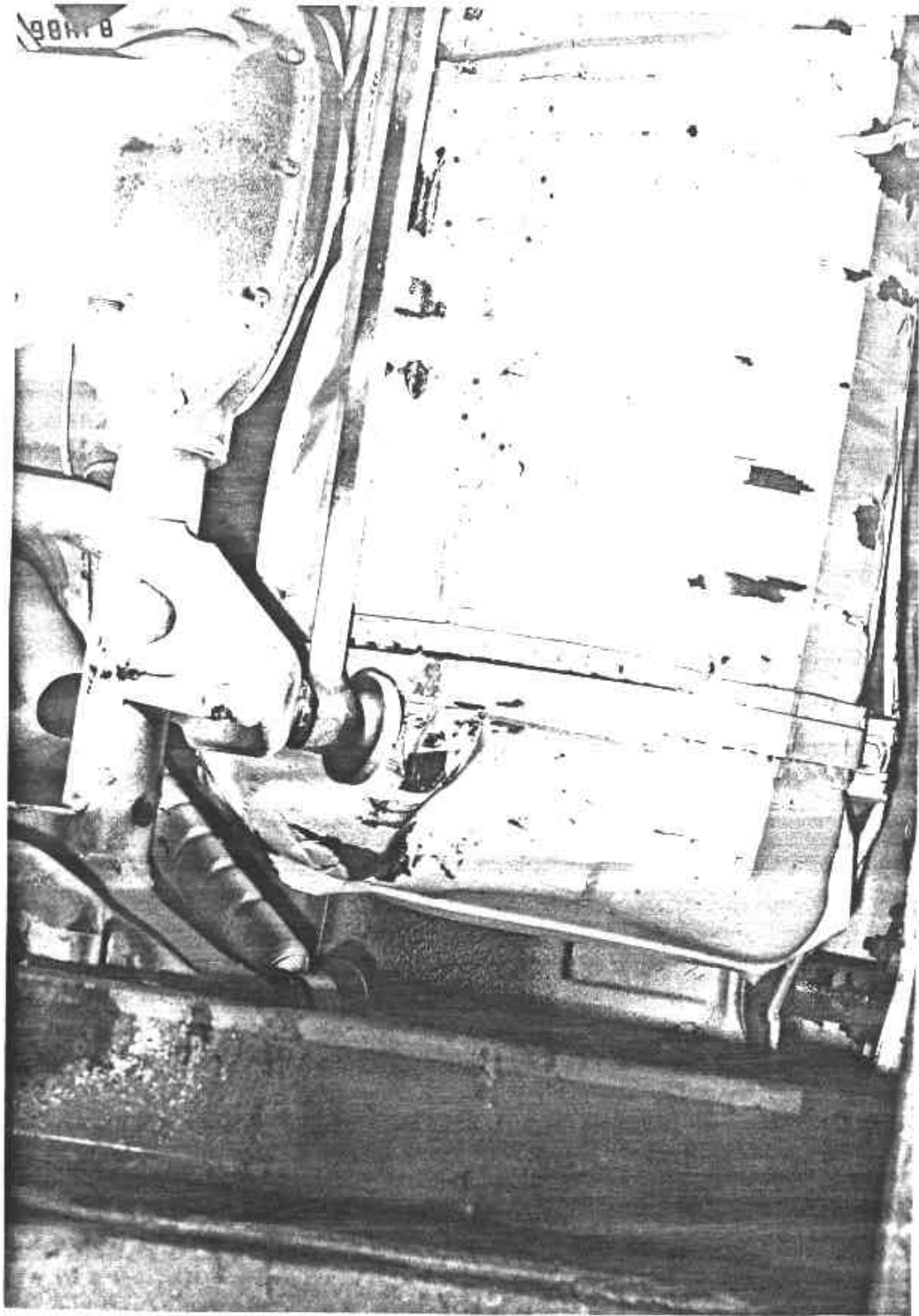
Figure 4-6. Post-test View of Fuel Tank - 1978 Chevrolet Chevette Four-door Hatchback Sedan - NHTSA 780112.
